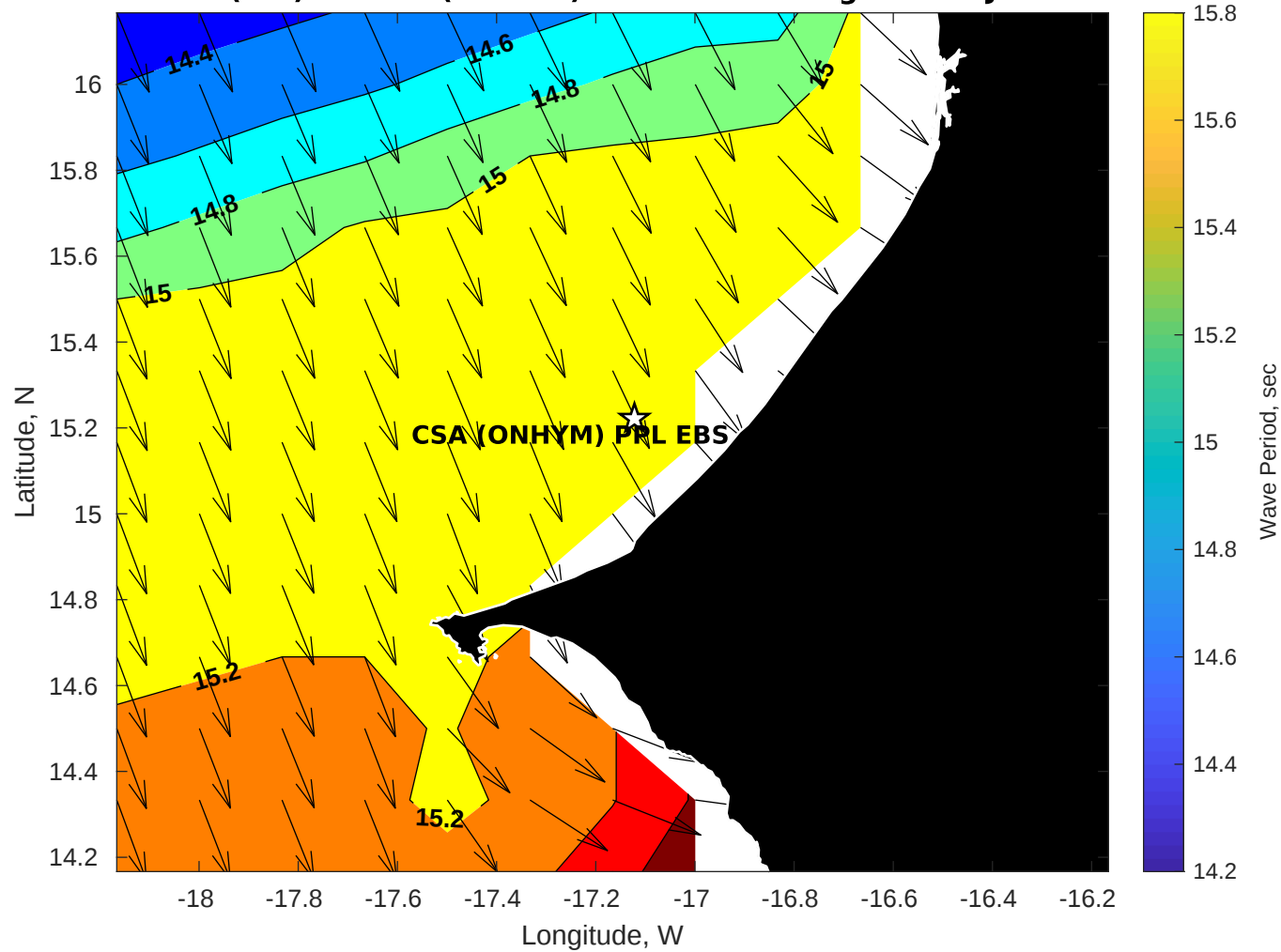
GFS Wave Period (sec) for CSA (ONHYM) PPL EBS - Senegal at 24-Jan-2026 09:00:00
