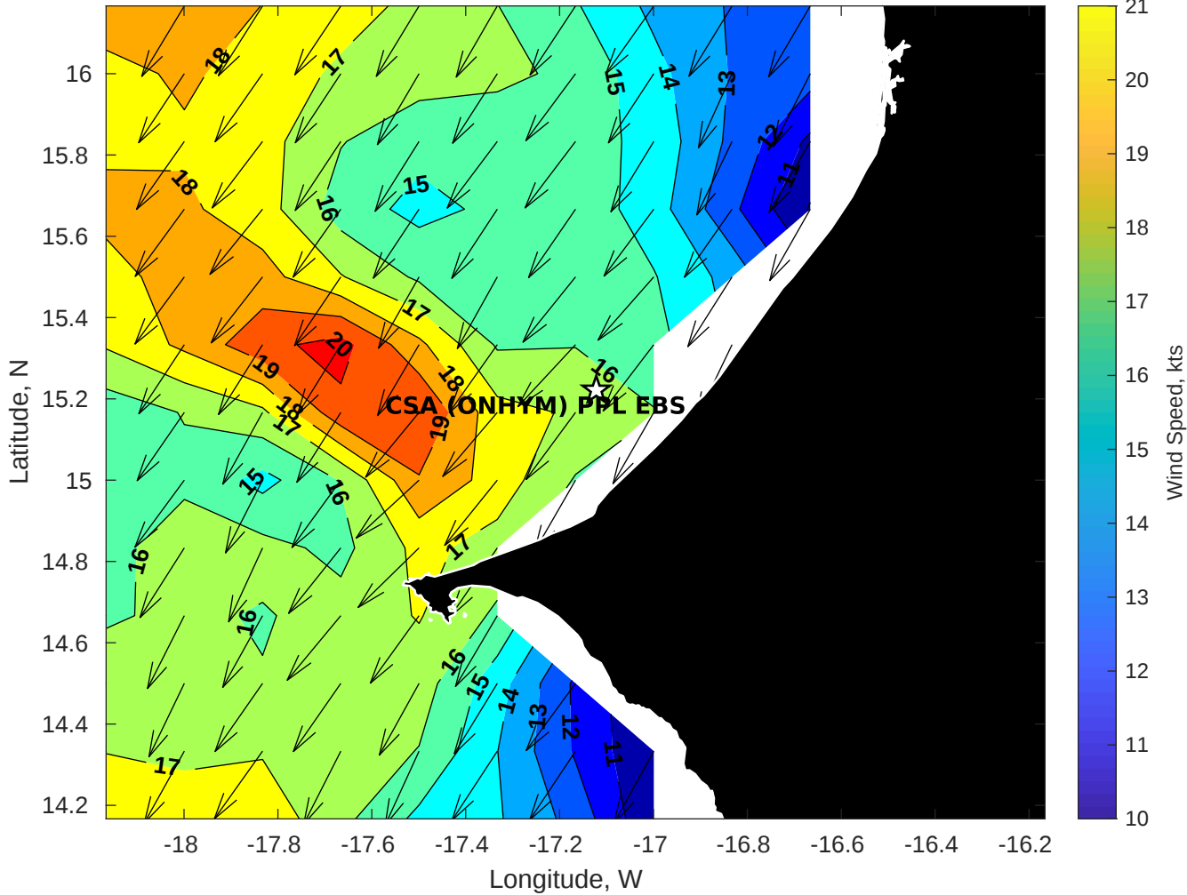
GFS Winds (kts) for CSA (ONHYM) PPL EBS - Senegal at 24-Jan-2026 09:00:00
