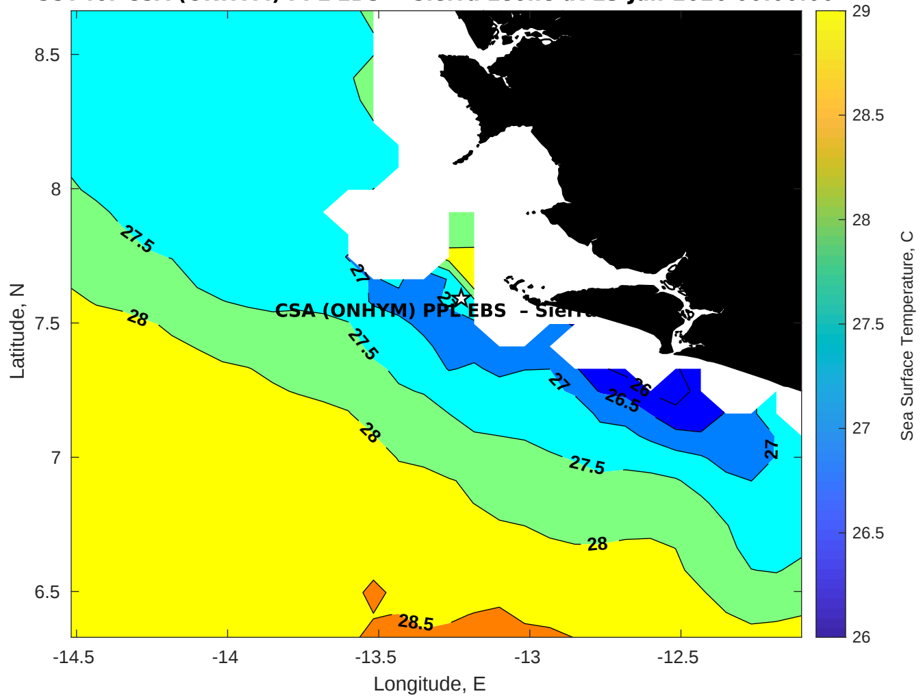
SST for CSA (ONHYM) PPL EBS - Sierra Leone at 23-Jan-2026 00:00:00
