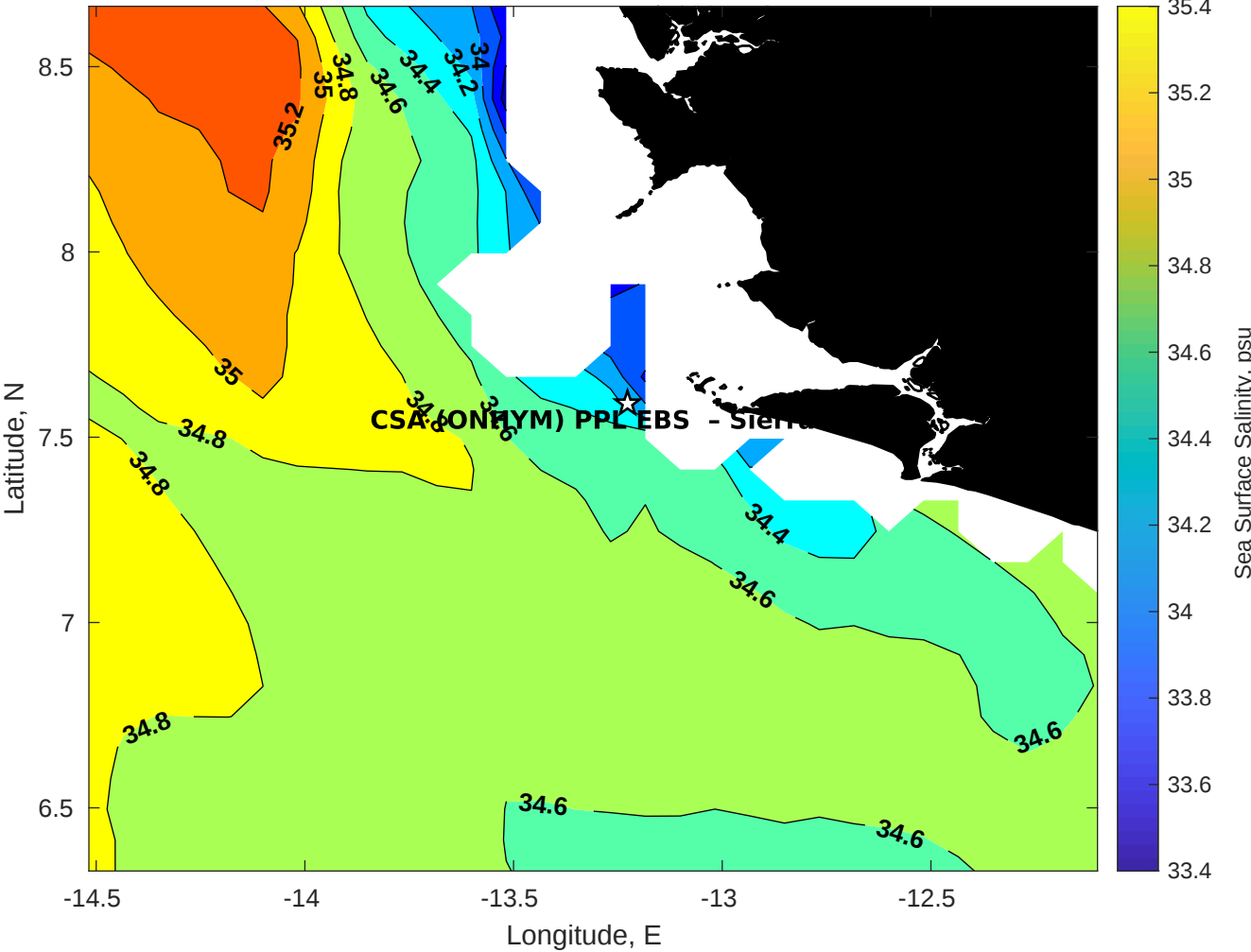
Surface Salinity for CSA (ONHYM) PPL EBS - Sierra Leone at 23-Jan-2026 00:00:00
