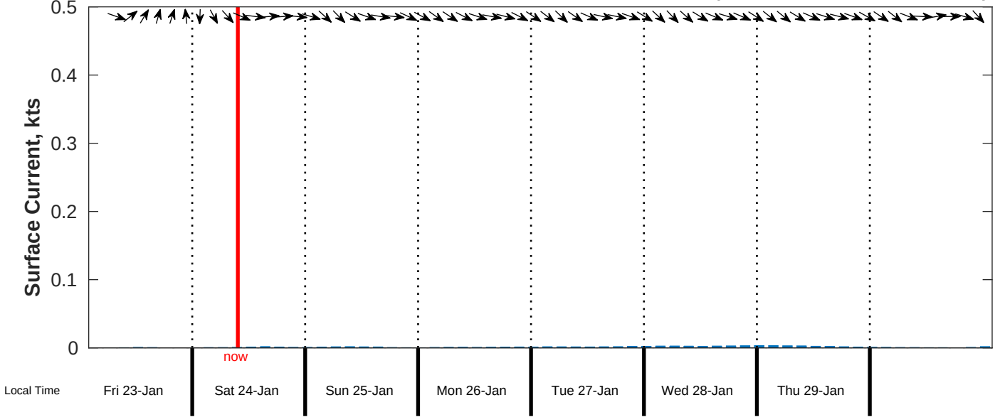
Surface Current Forecast for CSA (ONHYM) PPL EBS - Sierra Leone from 23-Jan-2026 00:00:00 to 31-Jan-2026 00:00:00
