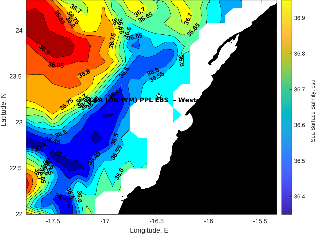
Surface Salinity for CSA (ONHYM) PPL EBS - Western Sahara at 23-Jan-2026 00:00:00
