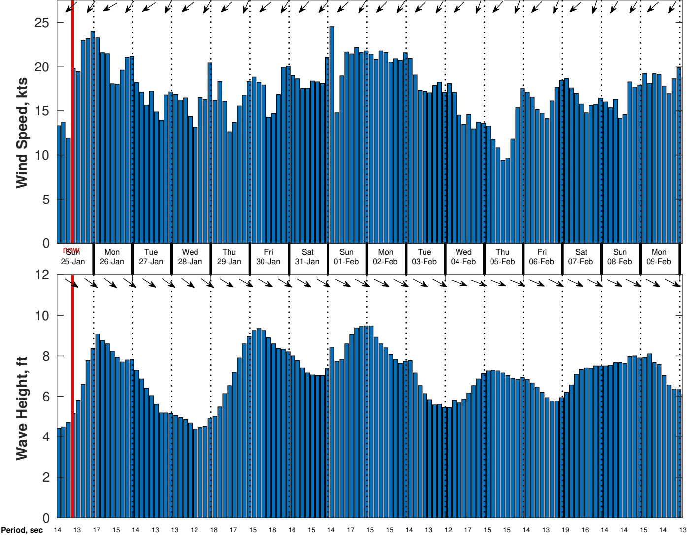
Wind & Wave Forecast for CSA (ONHYM) PPL EBS - Western Sahara from 24-Jan-2026 01:00:00 to 09-Feb-2026 01:00:00
