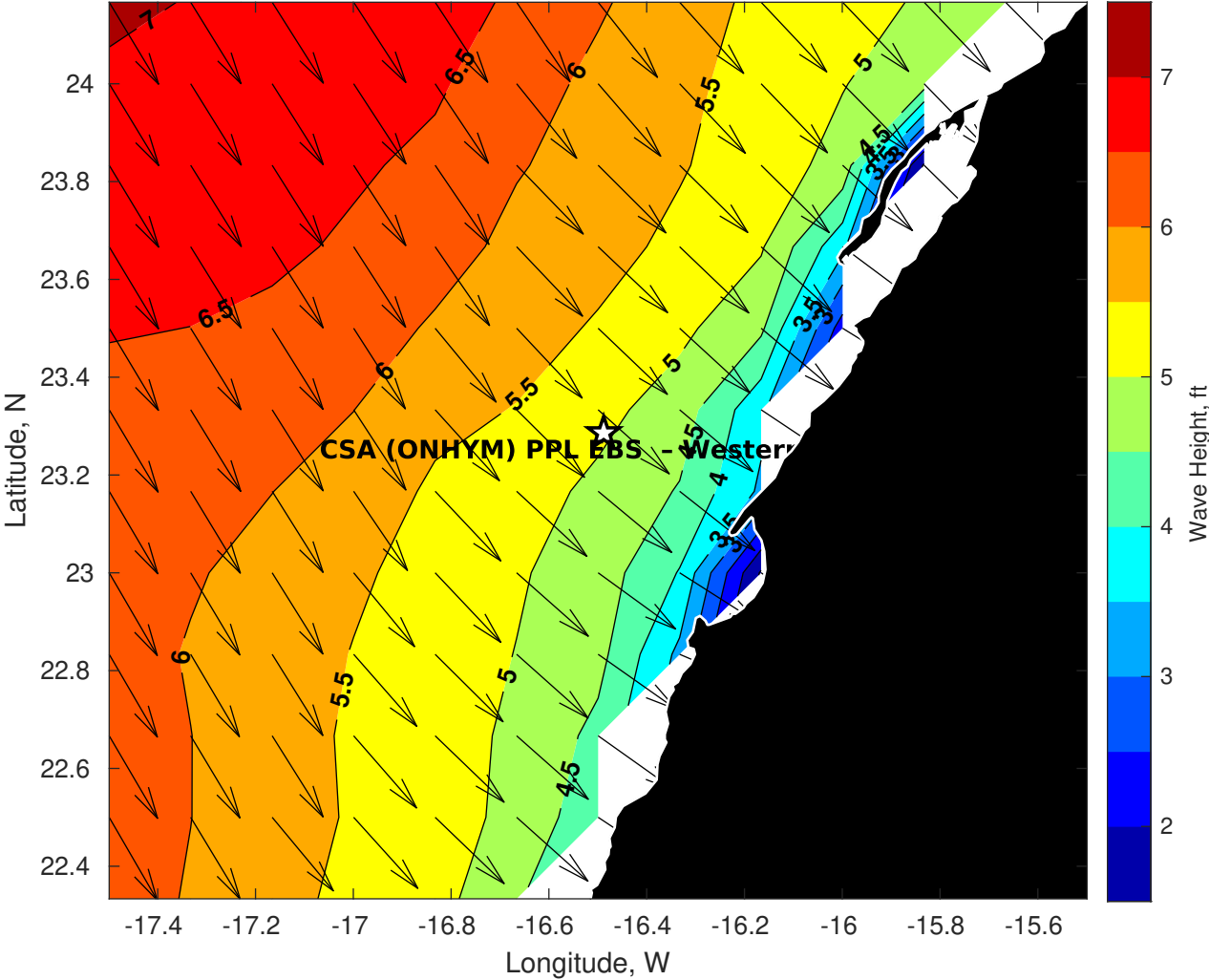
GFS Wave Height (ft) for CSA (ONHYM) PPL EBS - Western Sahara at 24-Jan-2026 09:00:00
