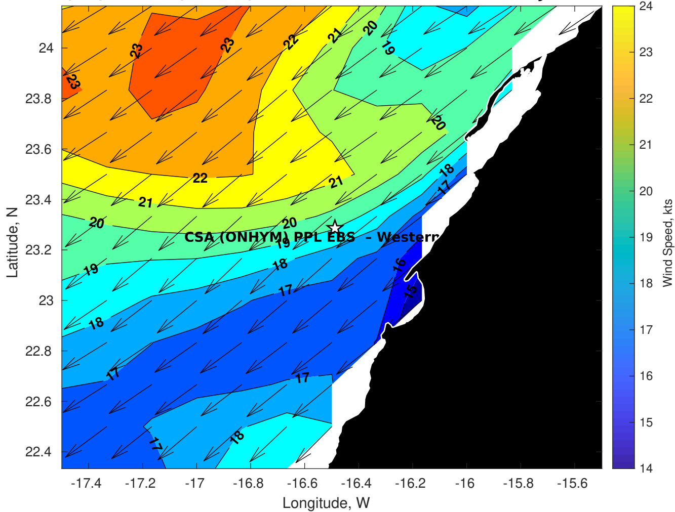
GFS Winds (kts) for CSA (ONHYM) PPL EBS - Western Sahara at 24-Jan-2026 09:00:00
