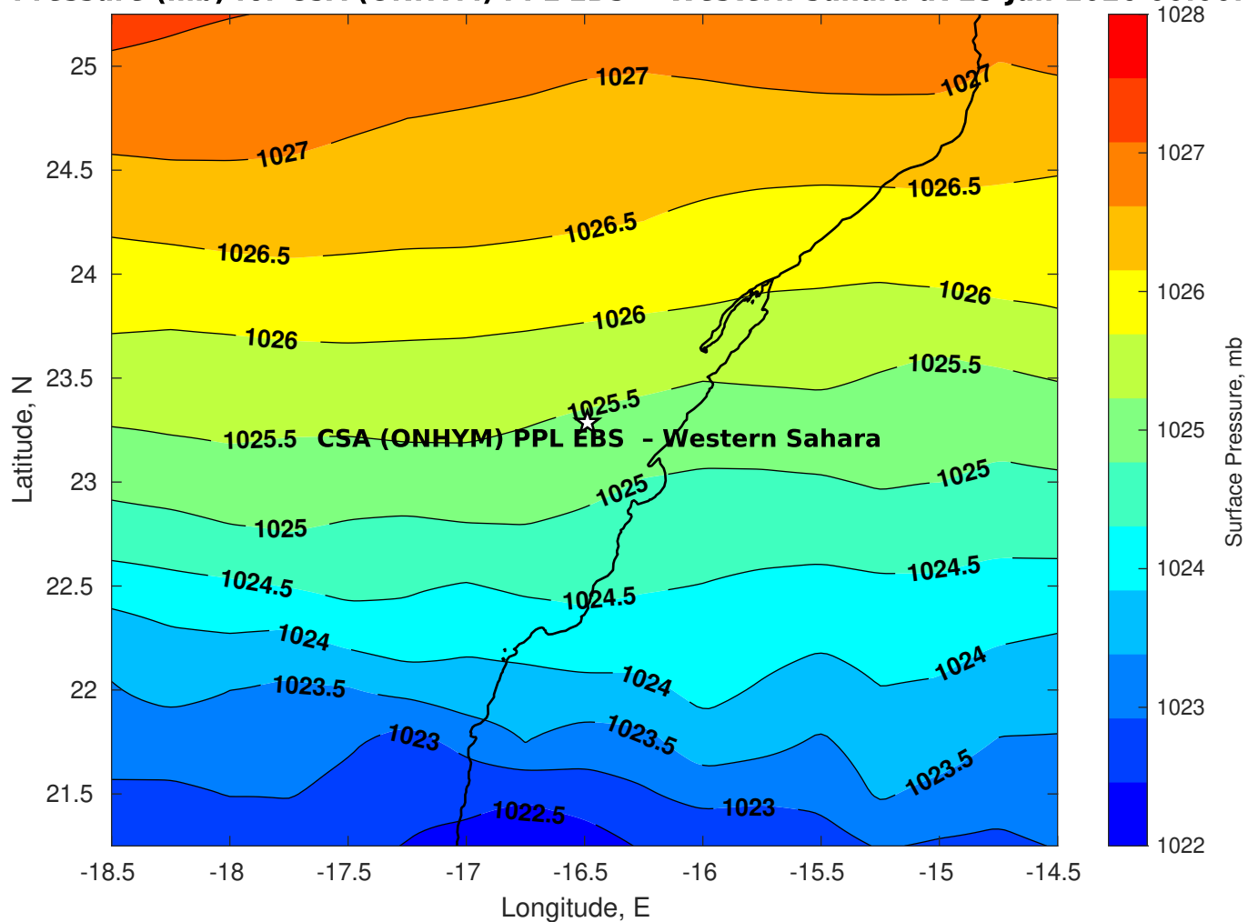
Surface Pressure (mb) for CSA (ONHYM) PPL EBS - Western Sahara at 25-Jan-2026 00:00:00
