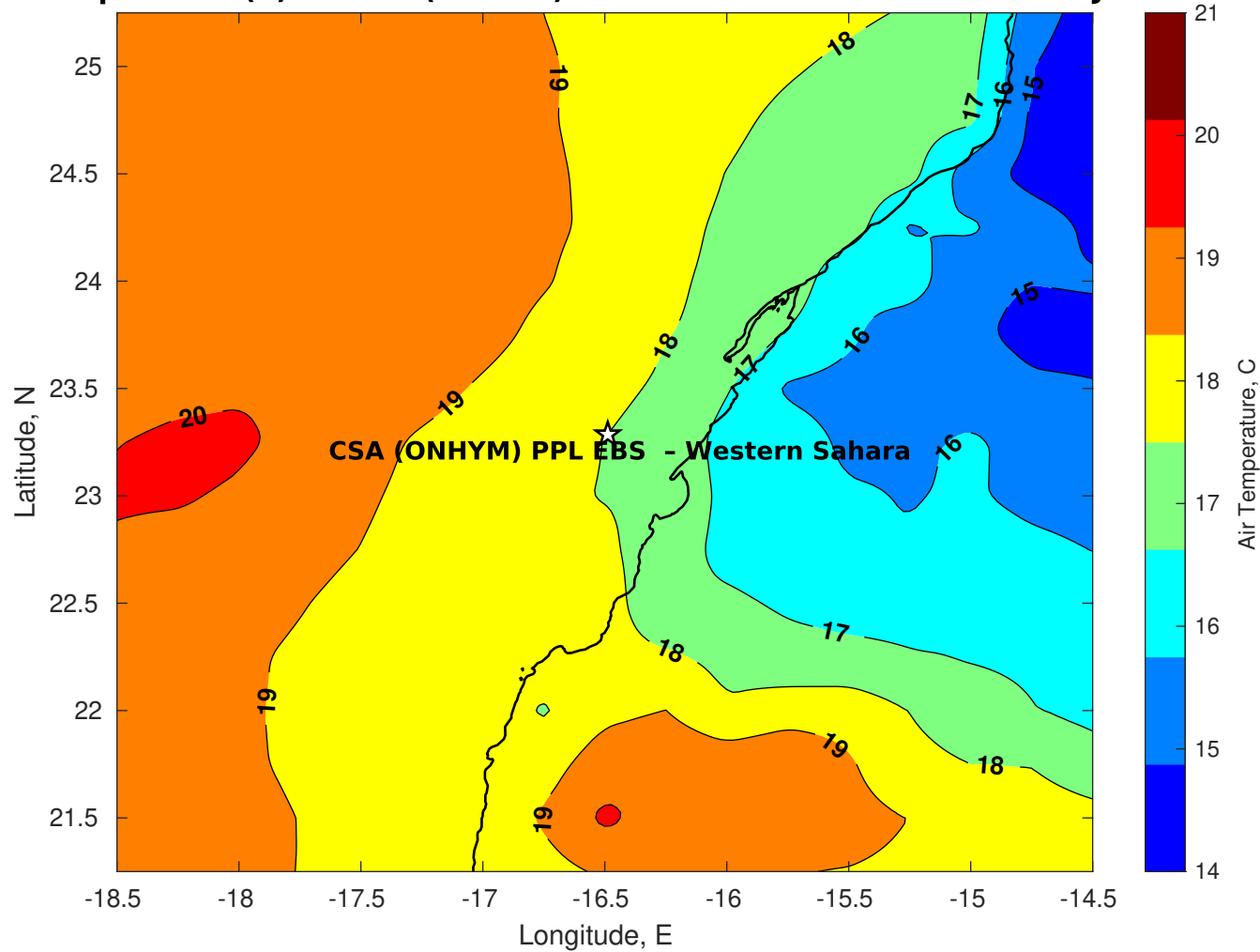
Air Temperature (C) for CSA (ONHYM) PPL EBS - Western Sahara at 24-Jan-2026
