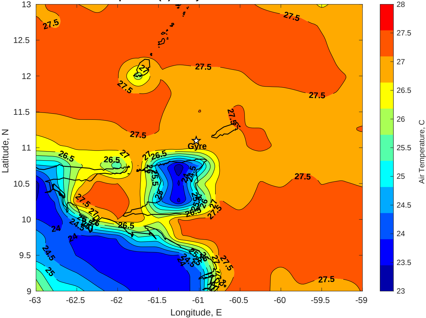
Air Temperature (C) for Gyre at 24-Jan-2026
