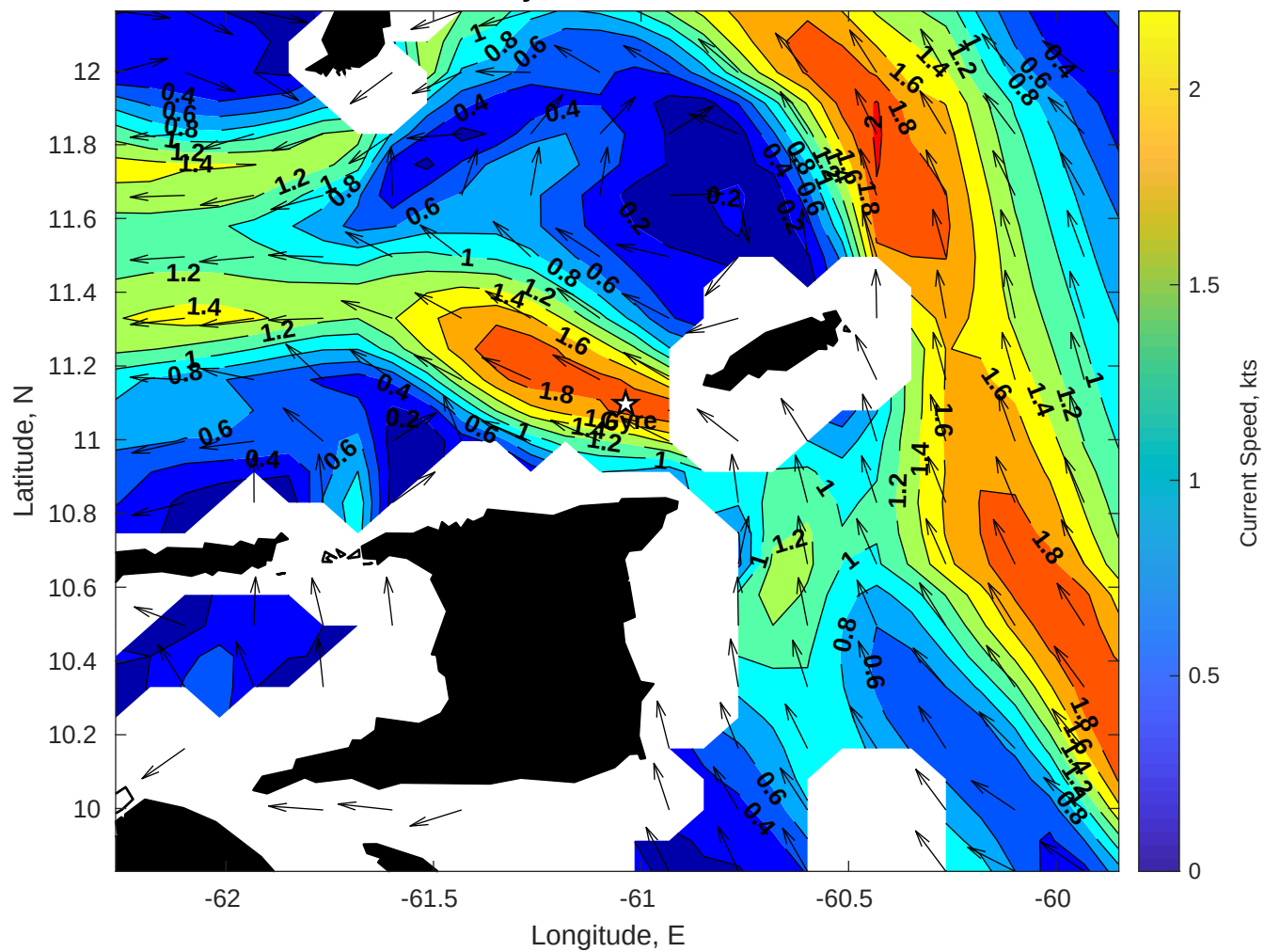
Surface Currents for Gyre at 23-Jan-2026 00:00:00
