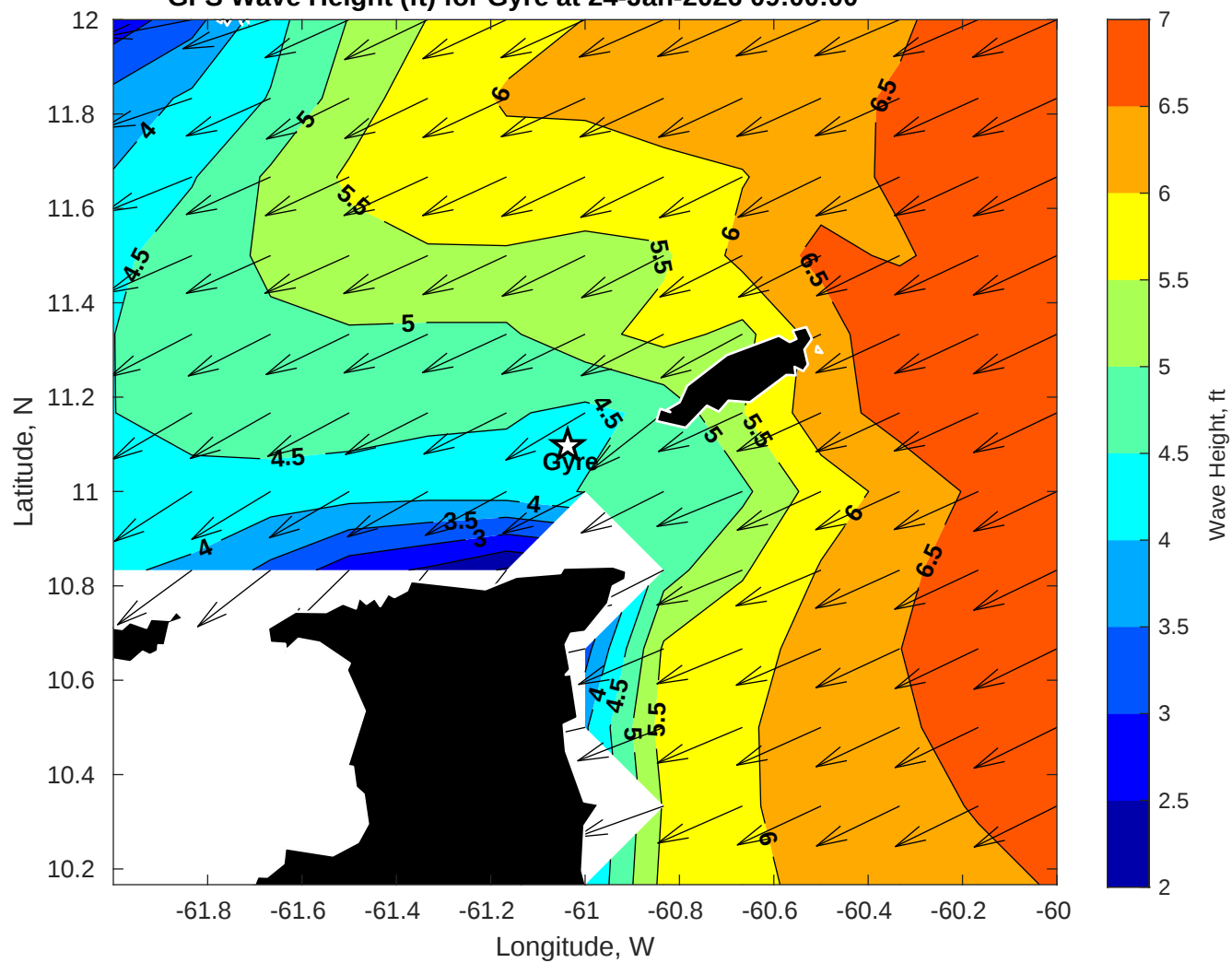
GFS Wave Height (ft) for Gyre at 24-Jan-2026 09:00:00
