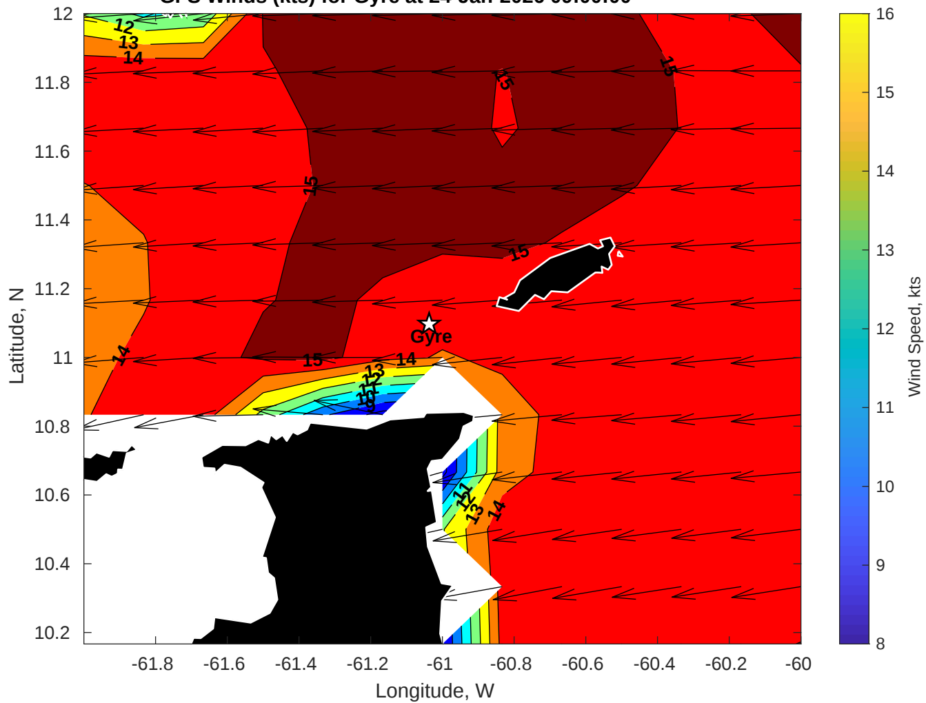
GFS Winds (kts) for Gyre at 24-Jan-2026 09:00:00
