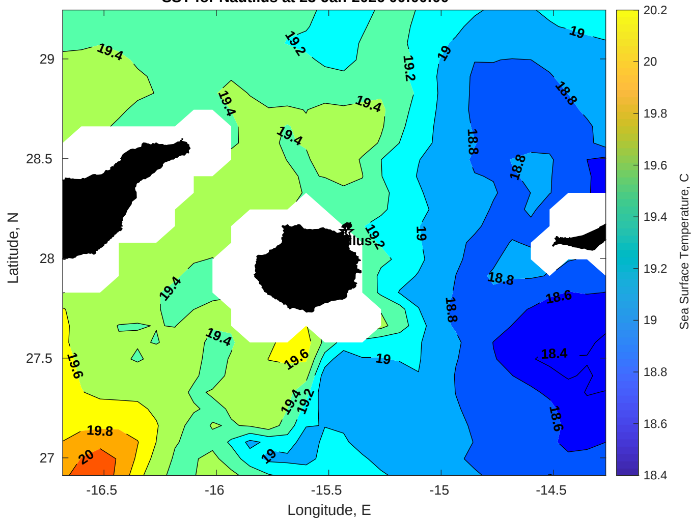
SST for Nautilus at 23-Jan-2026 00:00:00
