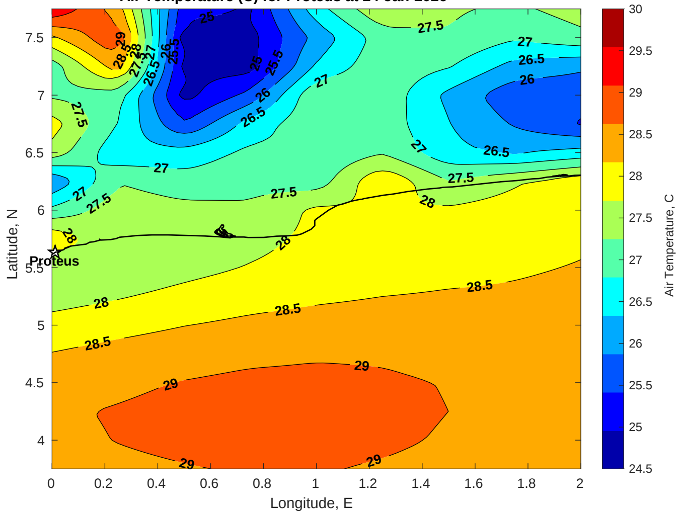
Air Temperature (C) for Proteus at 24-Jan-2026
