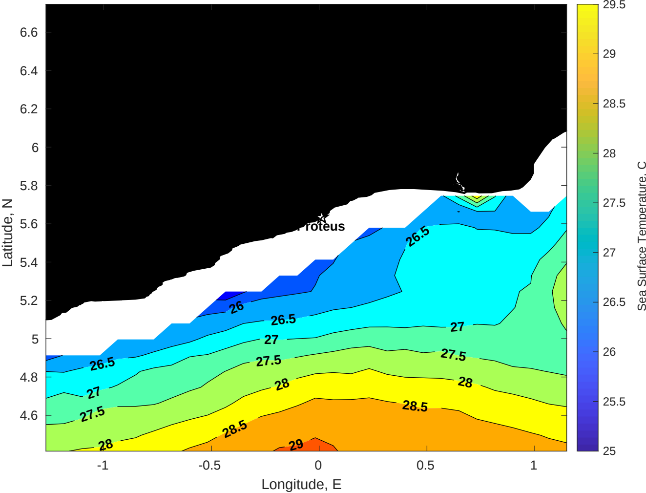
SST for Proteus at 23-Jan-2026 00:00:00
