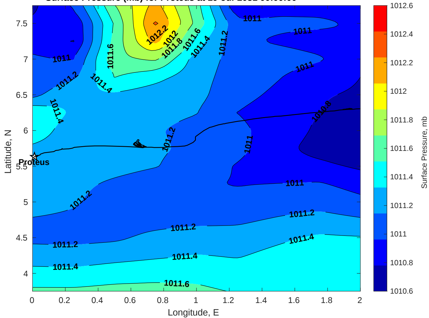
Surface Pressure (mb) for Proteus at 19-Jul-2031 00:00:00
