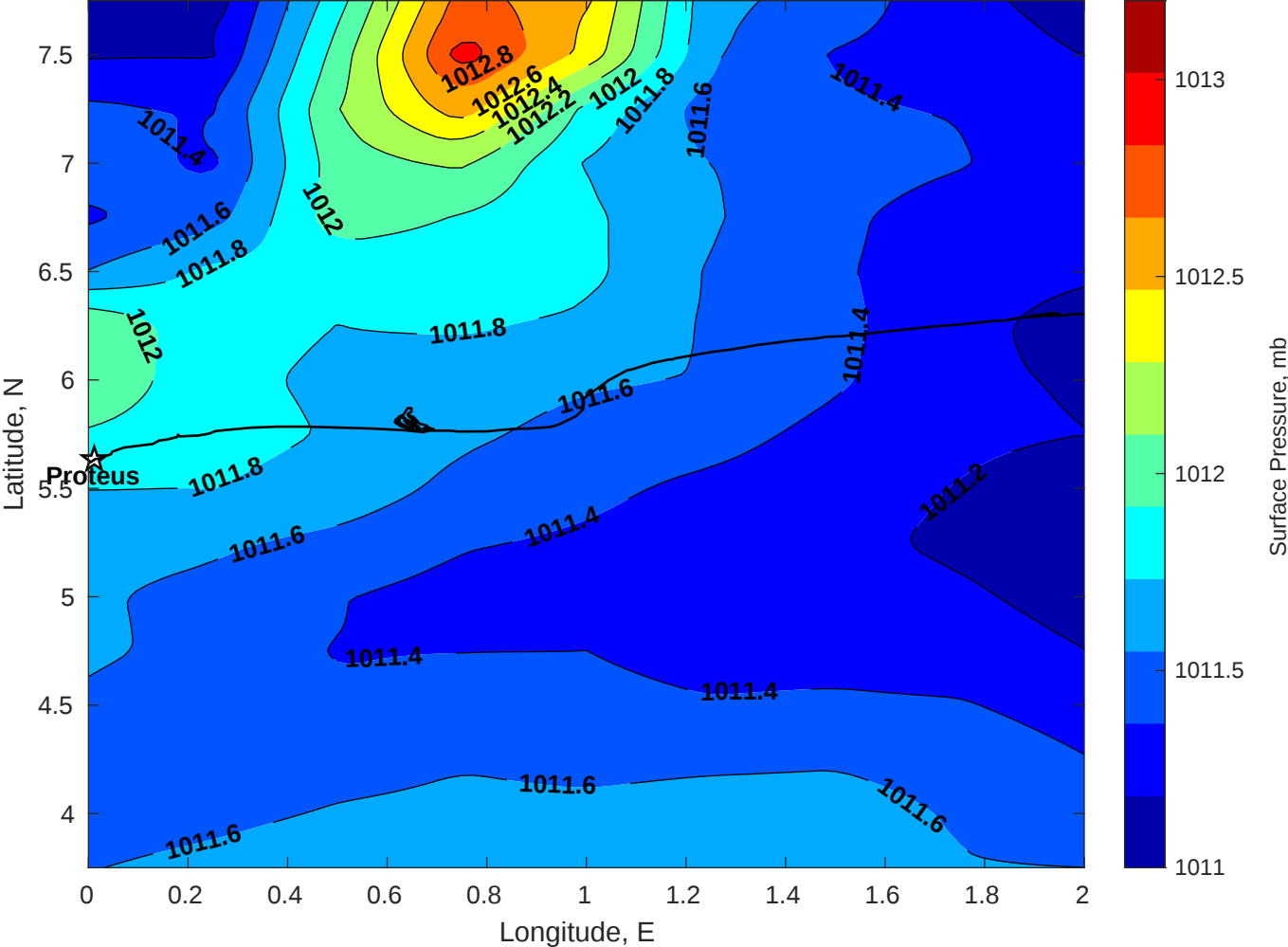
Surface Pressure (mb) for Proteus at 25-Jan-2026 00:00:00
