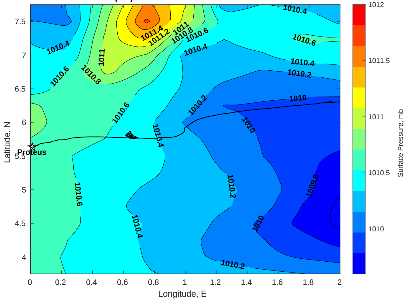
Surface Pressure (mb) for Proteus at 26-Jan-2026 00:00:00
