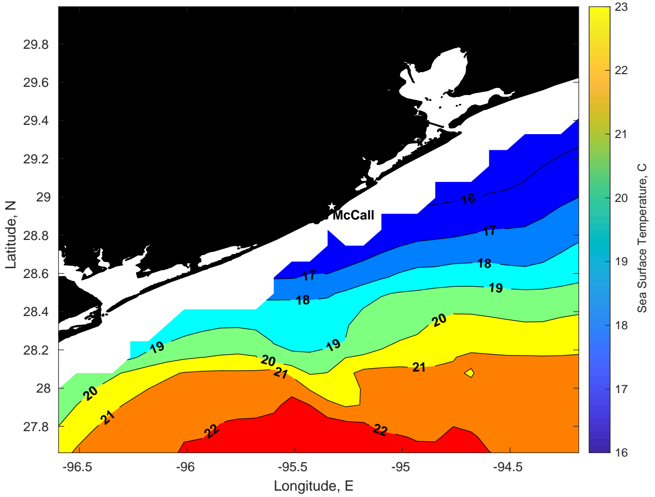
SST for Brooks McCall at 24-Jan-2026 00:00:00
