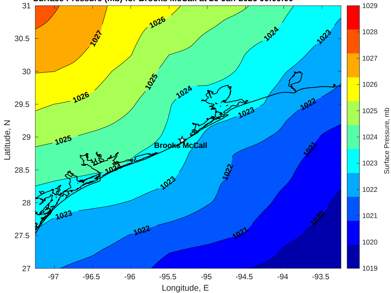
Surface Pressure (mb) for Brooks McCall at 26-Jan-2026 00:00:00
