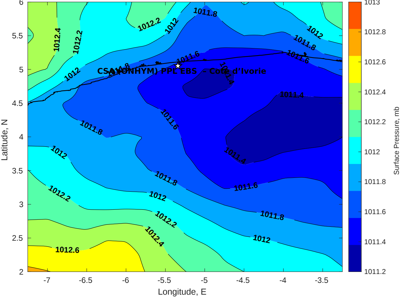
Surface Pressure (mb) for CSA (ONHYM) PPL EBS - Cote d'Ivoire at 26-Jan-2026 00:00:00
