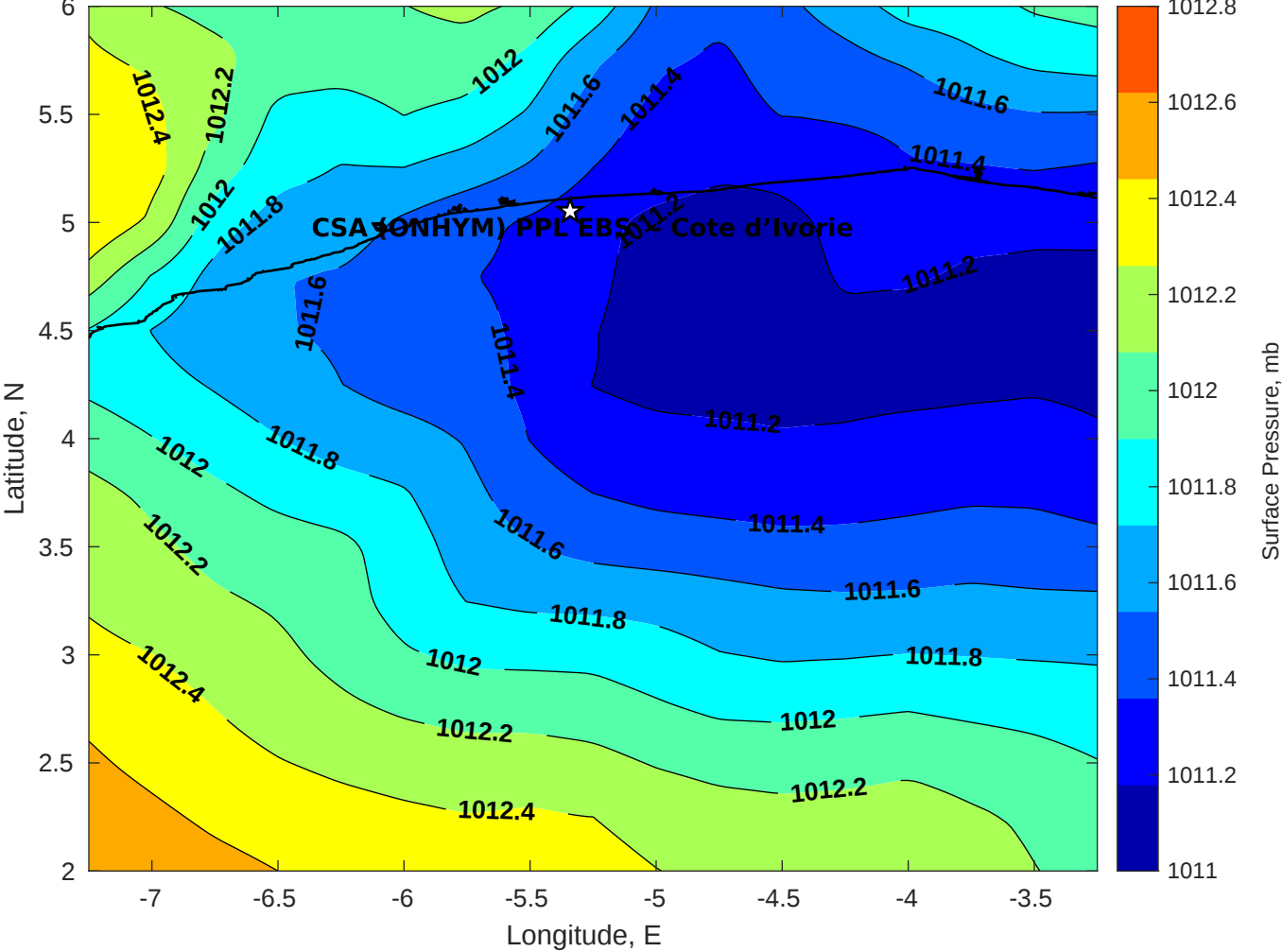
Surface Pressure (mb) for CSA (ONHYM) PPL EBS - Cote d'Ivoire at 27-Jan-2026 00:00:00
