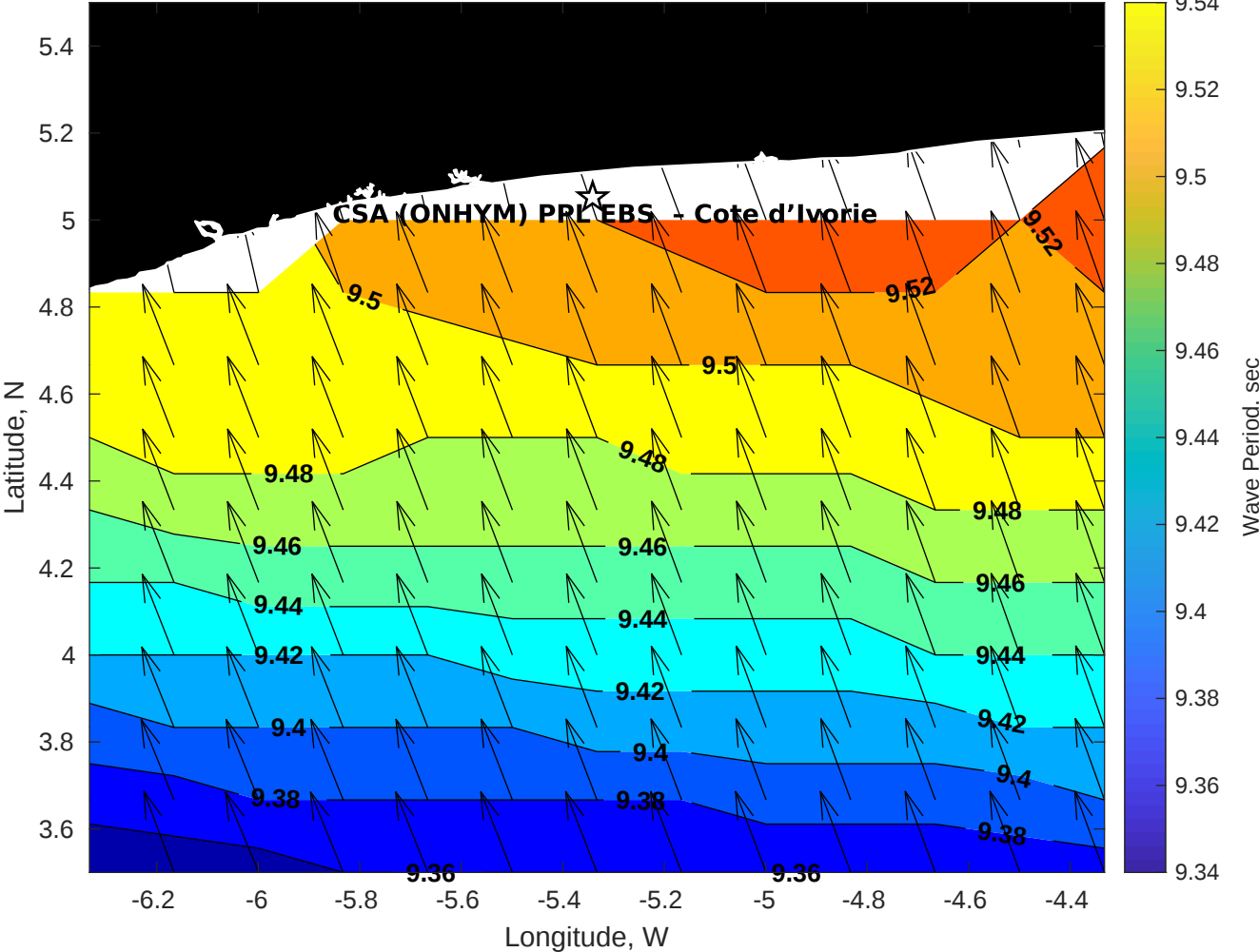
GFS Wave Period (sec) for CSA (ONHYM) PPL EBS - Cote d'Ivoire at 25-Jan-2026 09:00:00
