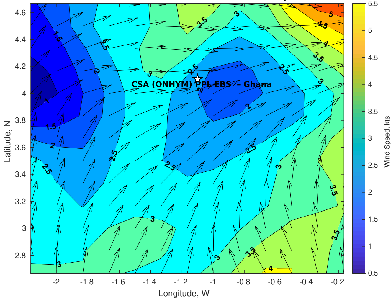
GFS Winds (kts) for CSA (ONHYM) PPL EBS - Ghana at 25-Jan-2026 09:00:00
