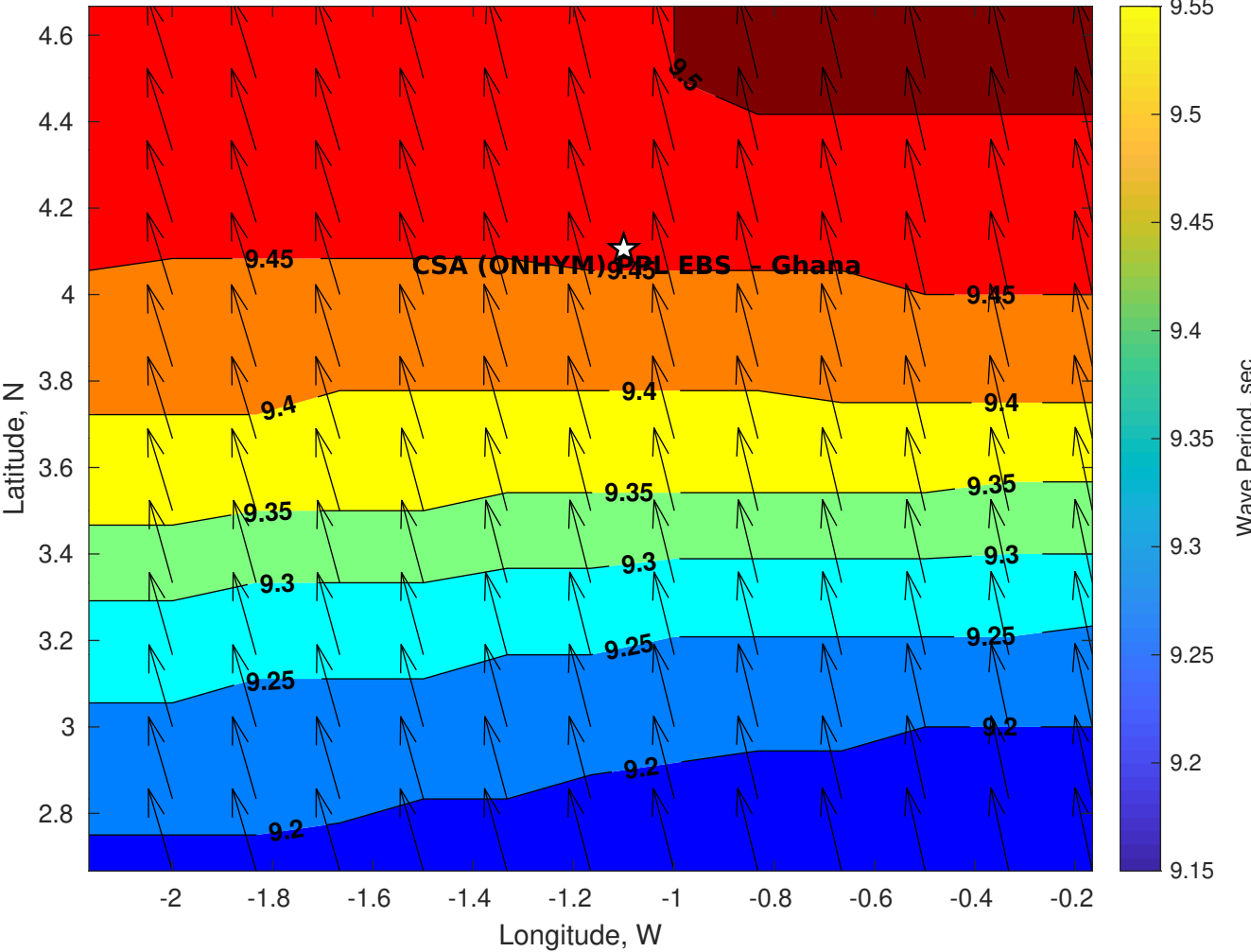
GFS Wave Period (sec) for CSA (ONHYM) PPL EBS - Ghana at 25-Jan-2026 09:00:00
