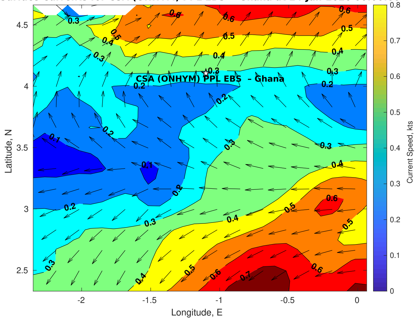
Surface Currents for CSA (ONHYM) PPL EBS - Ghana at 24-Jan-2026 00:00:00
