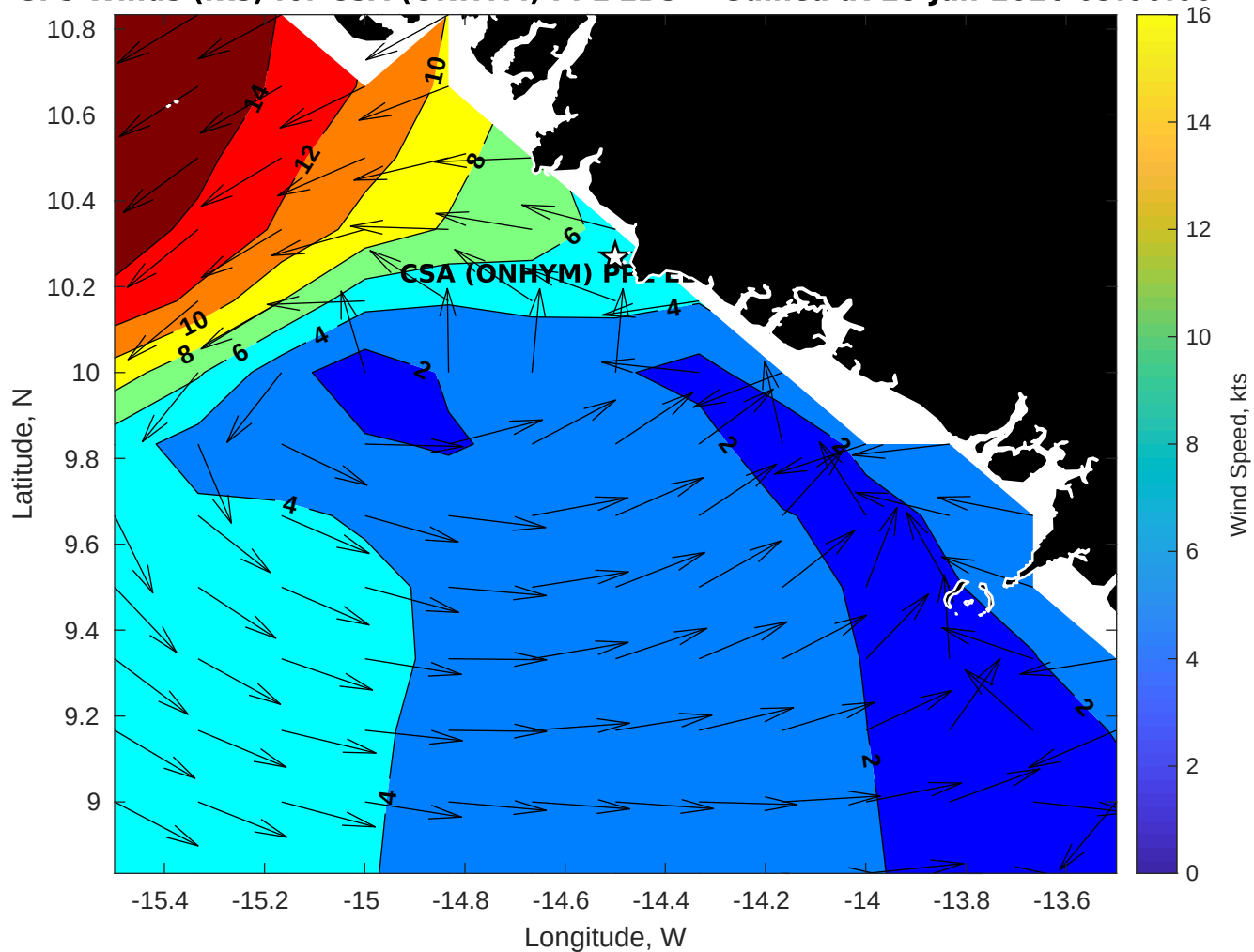
GFS Winds (kts) for CSA (ONHYM) PPL EBS - Guinea at 25-Jan-2026 09:00:00
