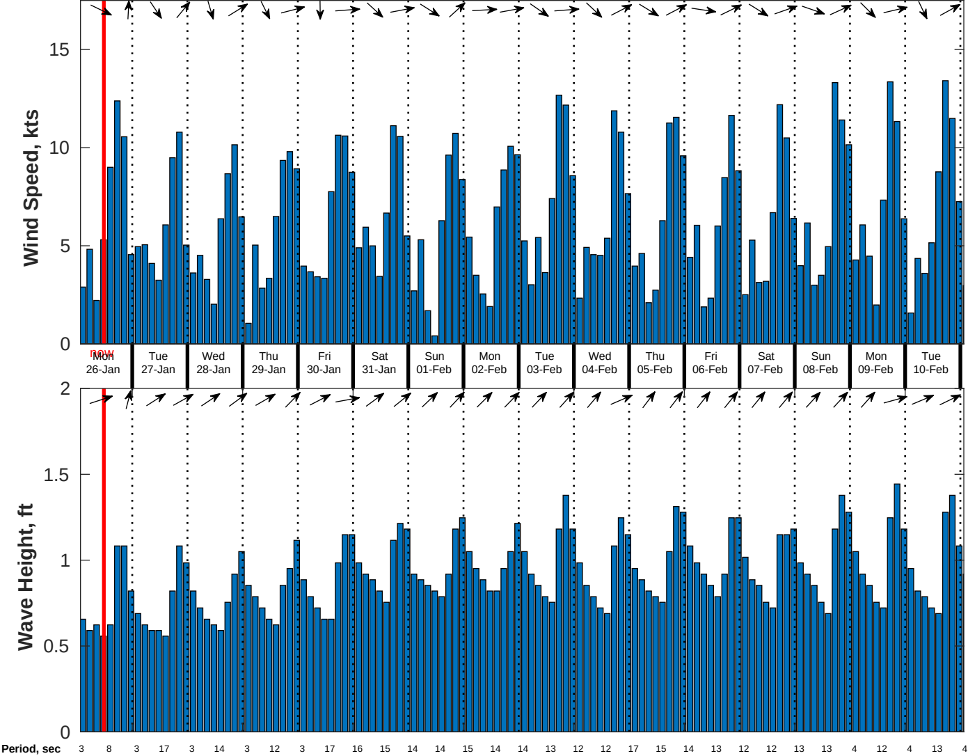
Wind & Wave Forecast for CSA (ONHYM) PPL EBS - Guinea from 25-Jan-2026 01:00:00 to 10-Feb-2026 01:00:00
