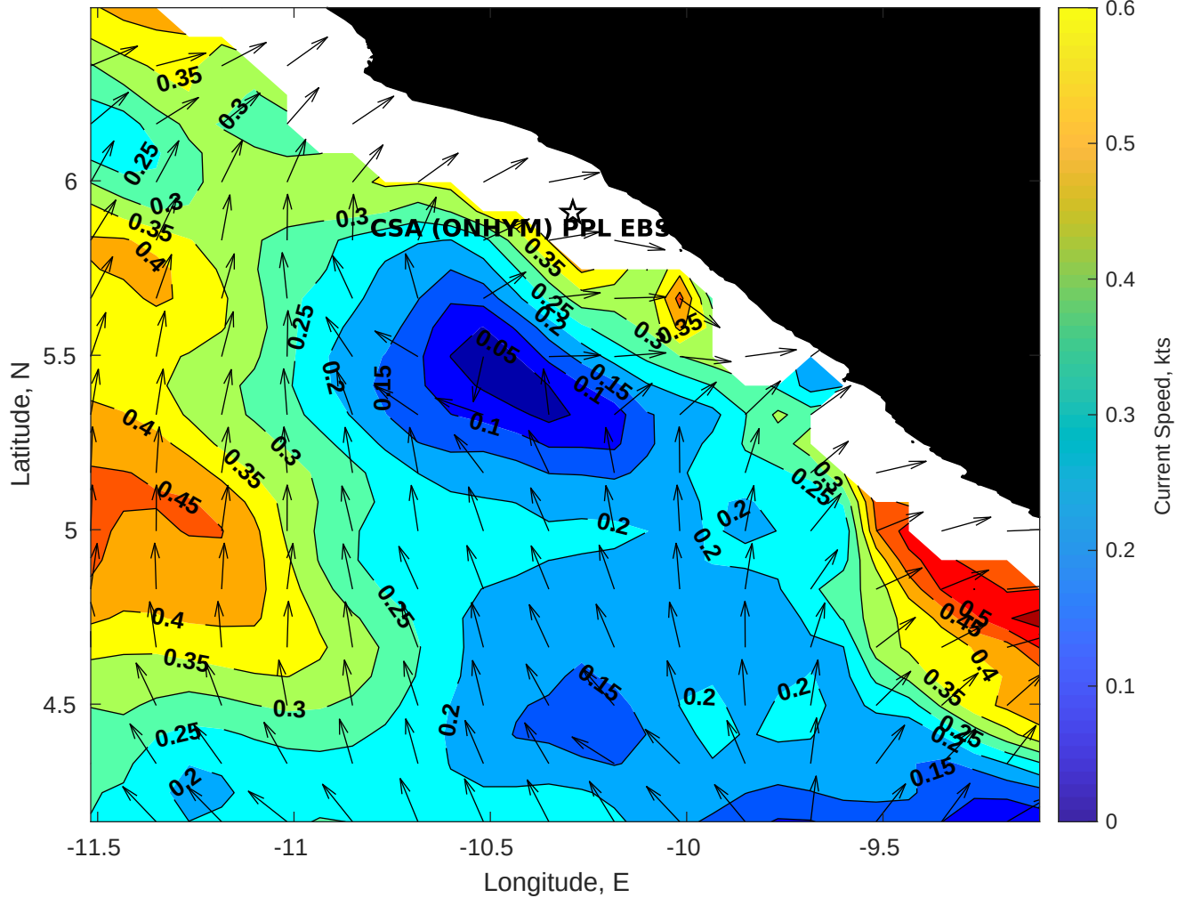
Surface Currents for CSA (ONHYM) PPL EBS - Liberia at 24-Jan-2026 00:00:00
