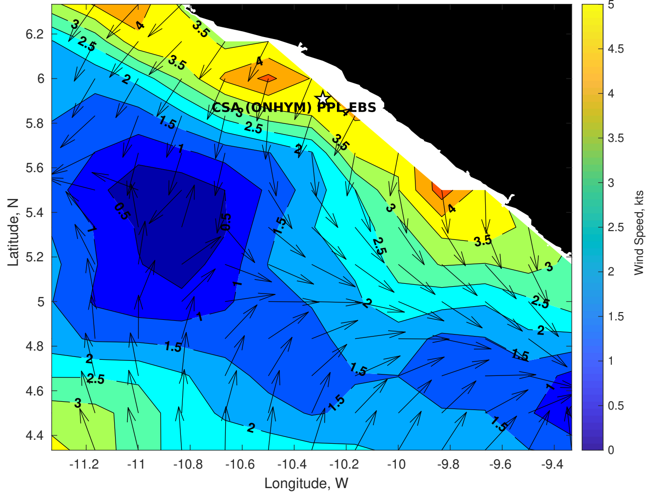
GFS Winds (kts) for CSA (ONHYM) PPL EBS - Liberia at 25-Jan-2026 09:00:00
