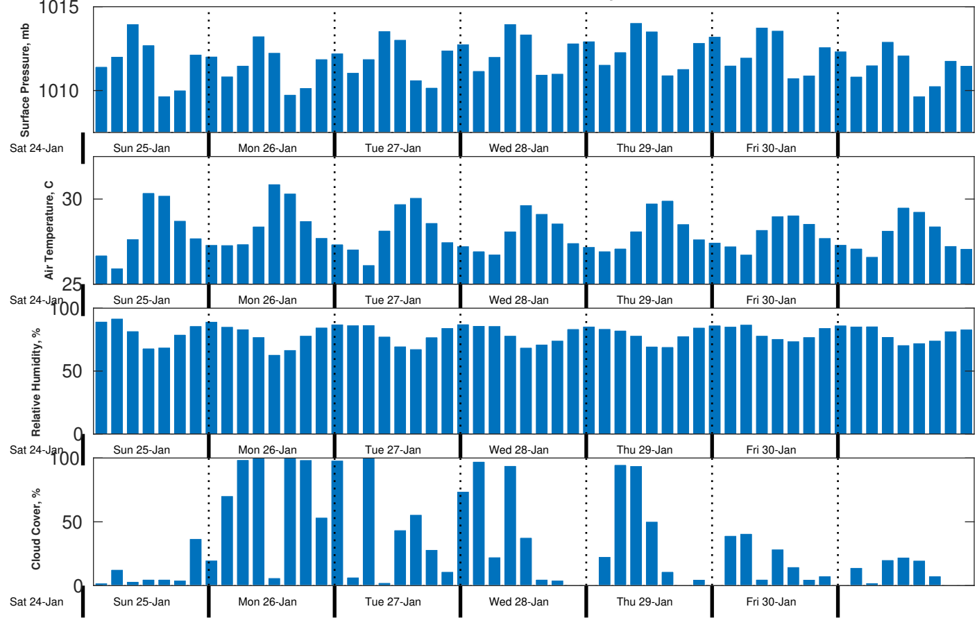
Met Forecast for CSA (ONHYM) PPL EBS - Liberia from 25-Jan-2026 00:00:00 to 01-Feb-2026 00:00:00
