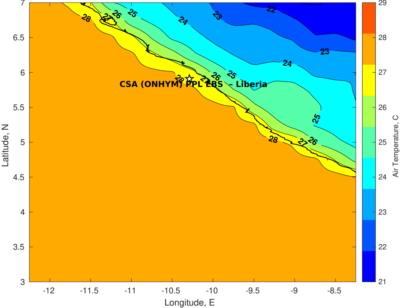
Air Temperature (C) for CSA (ONHYM) PPL EBS - Liberia at 25-Jan-2026
