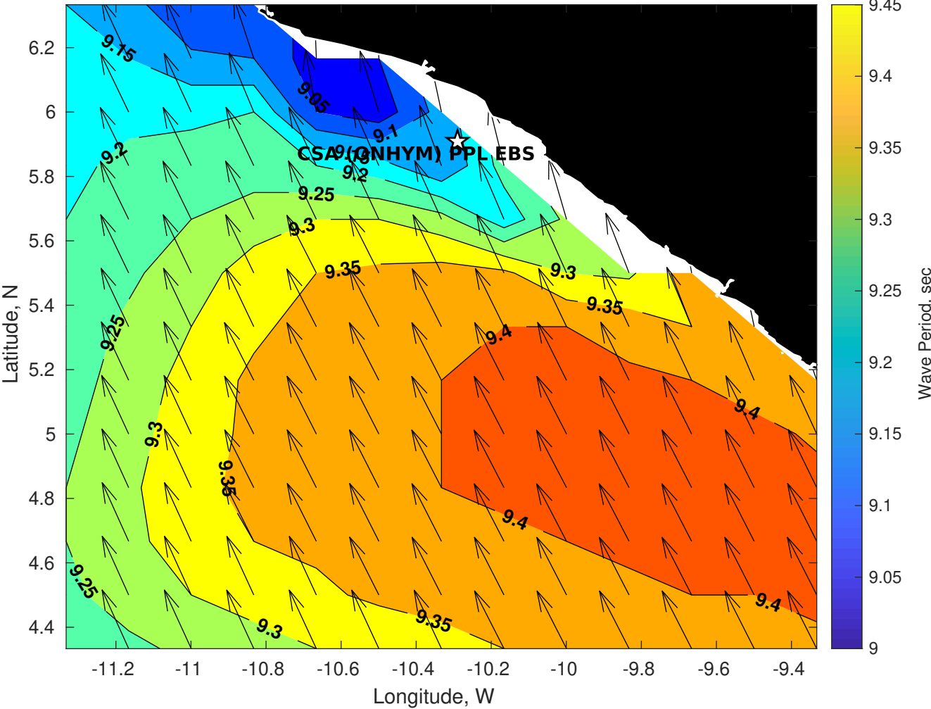
GFS Wave Period (sec) for CSA (ONHYM) PPL EBS - Liberia at 25-Jan-2026 09:00:00
