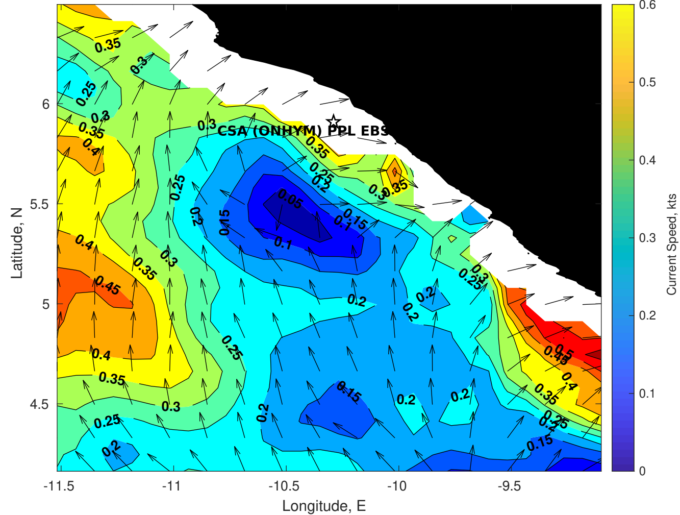
Surface Currents for CSA (ONHYM) PPL EBS - Liberia at 24-Jan-2026 00:00:00
