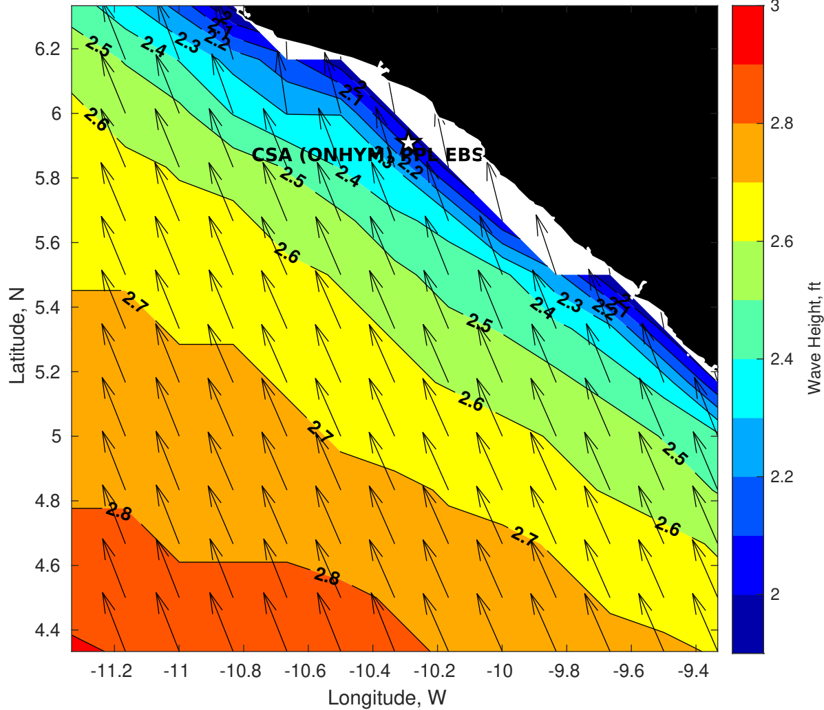
GFS Wave Height (ft) for CSA (ONHYM) PPL EBS - Liberia at 25-Jan-2026 09:00:00
