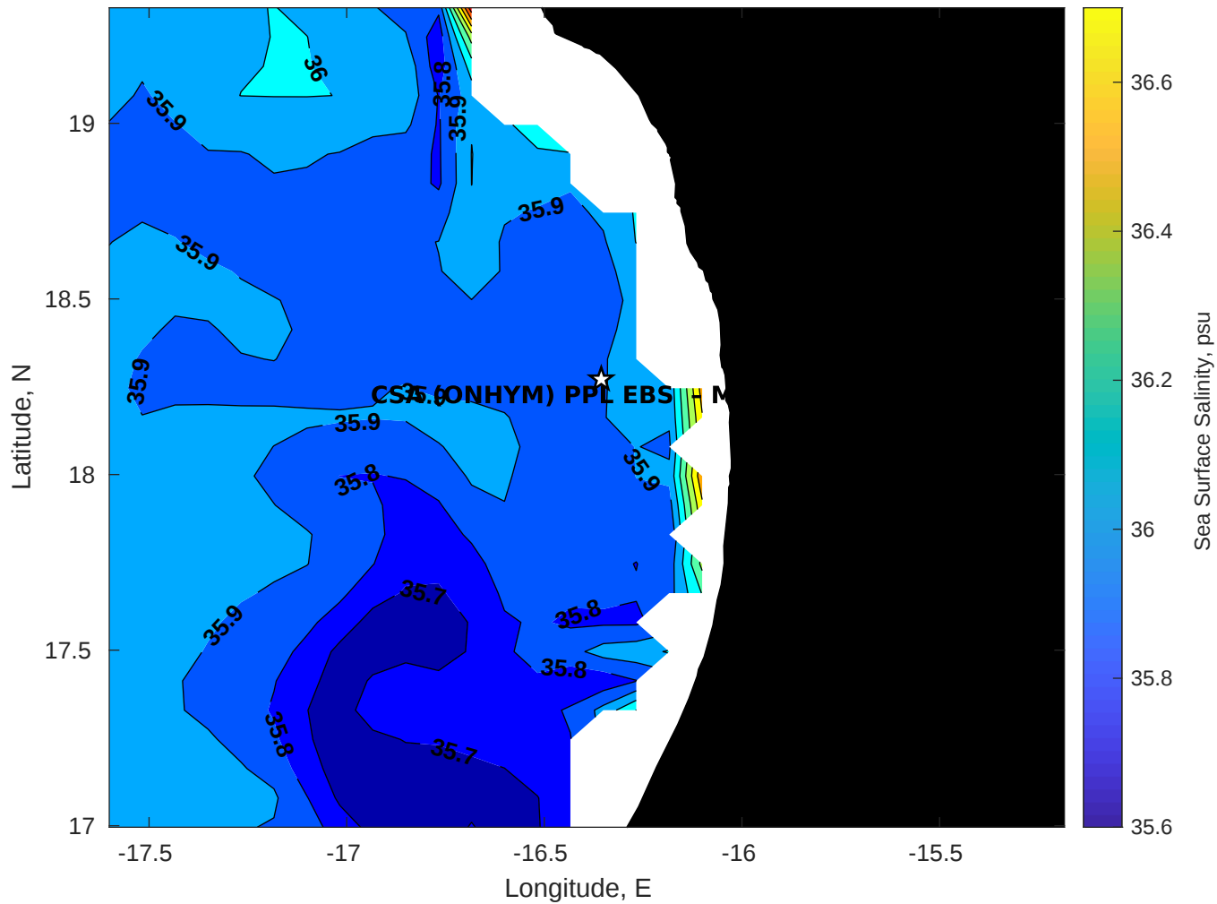
Surface Salinity for CSA (ONHYM) PPL EBS - Mauritania at 24-Jan-2026 00:00:00
