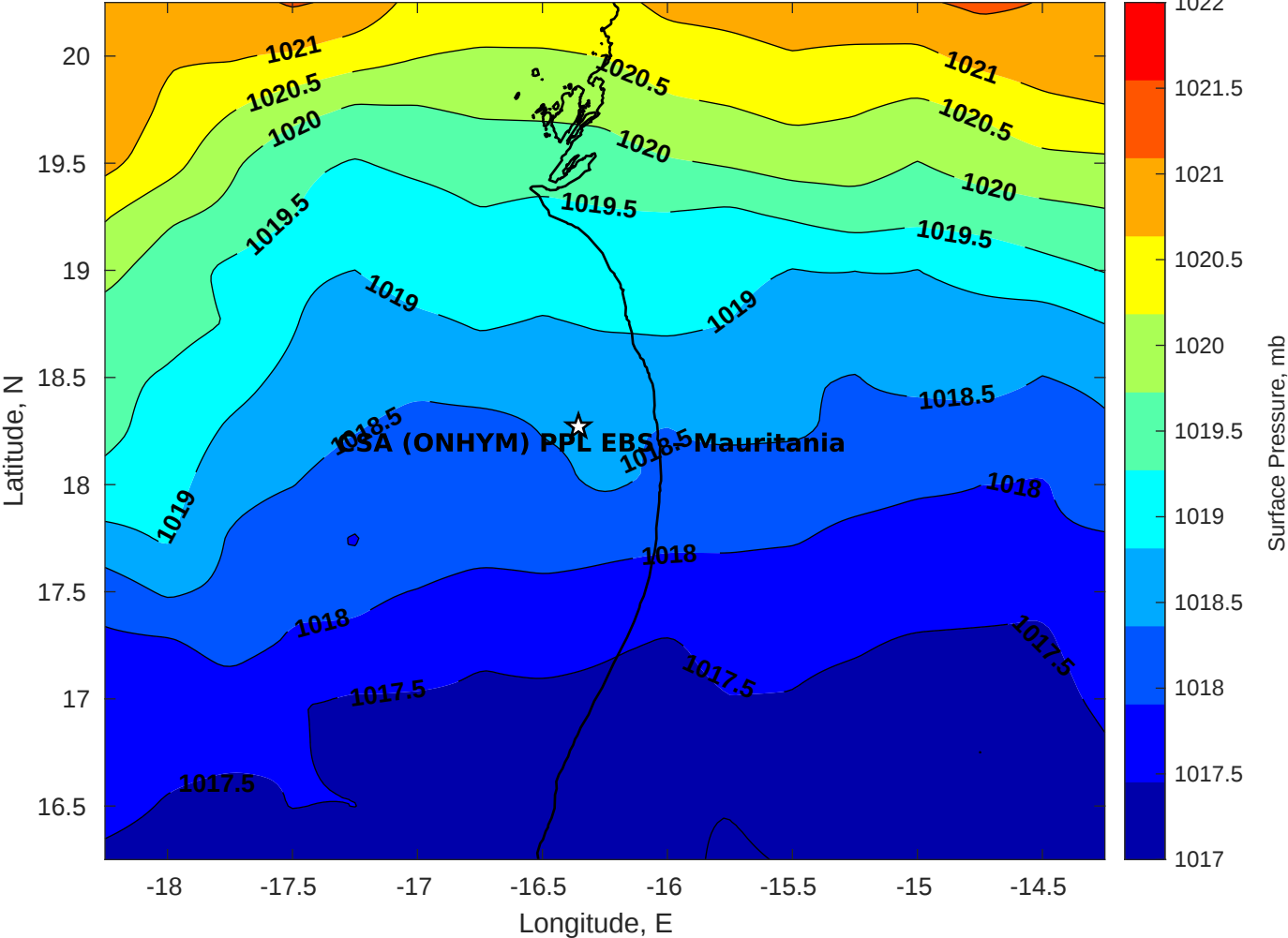
Surface Pressure (mb) for CSA (ONHYM) PPL EBS - Mauritania at 25-Jan-2026 00:00:00
