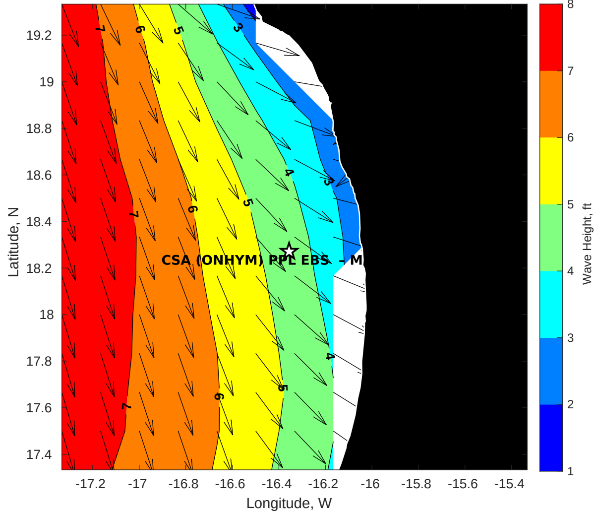
GFS Wave Height (ft) for CSA (ONHYM) PPL EBS - Mauritania at 25-Jan-2026 09:00:00
