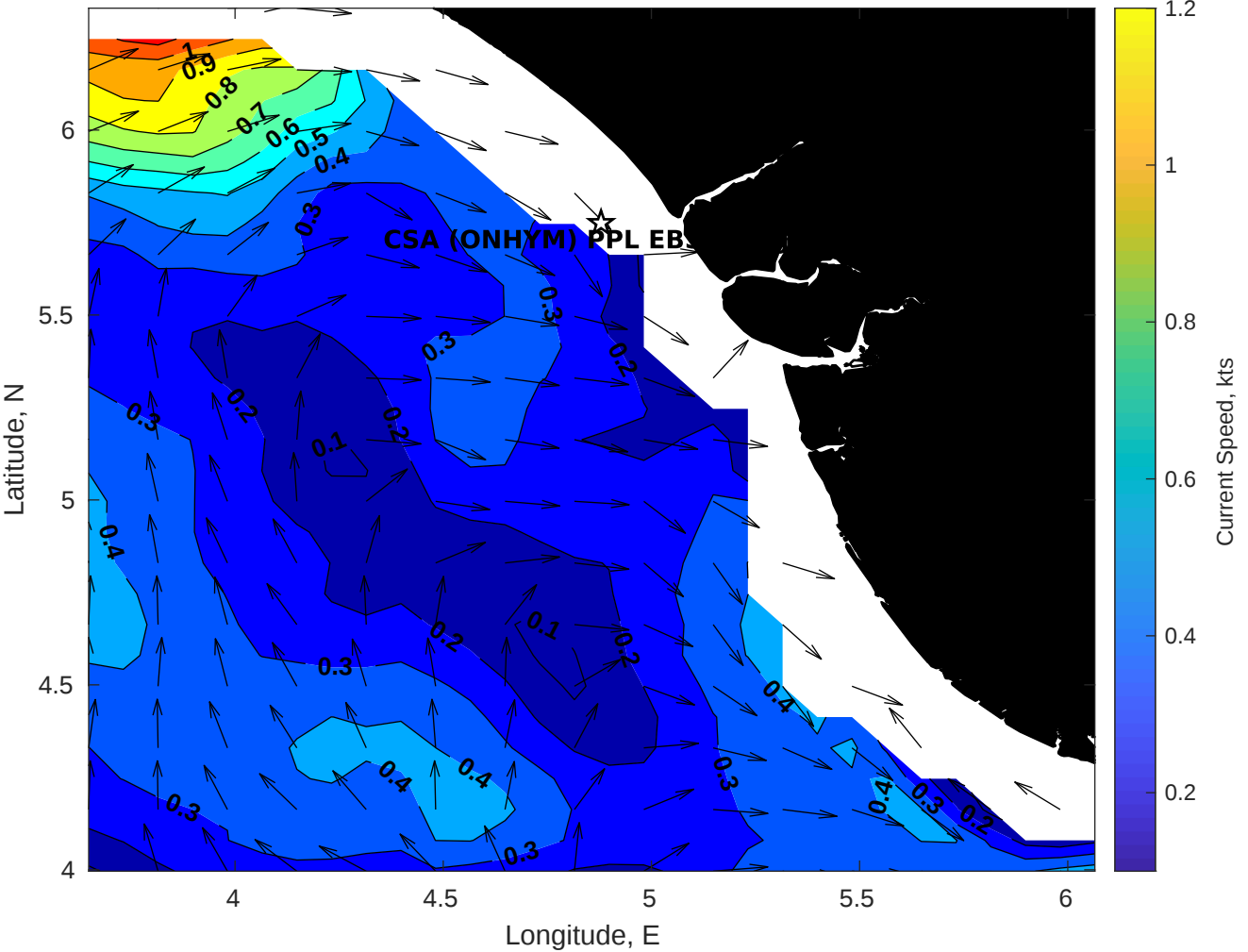
Surface Currents for CSA (ONHYM) PPL EBS - Nigeria at 24-Jan-2026 00:00:00
