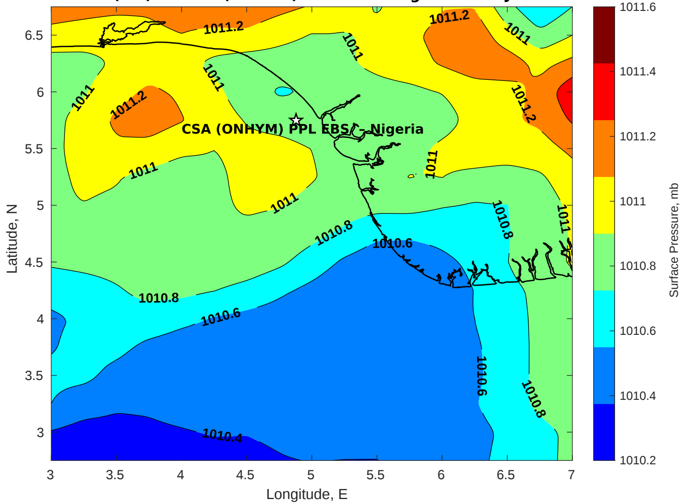
Surface Pressure (mb) for CSA (ONHYM) PPL EBS - Nigeria at 26-Jan-2026 06:00:00
