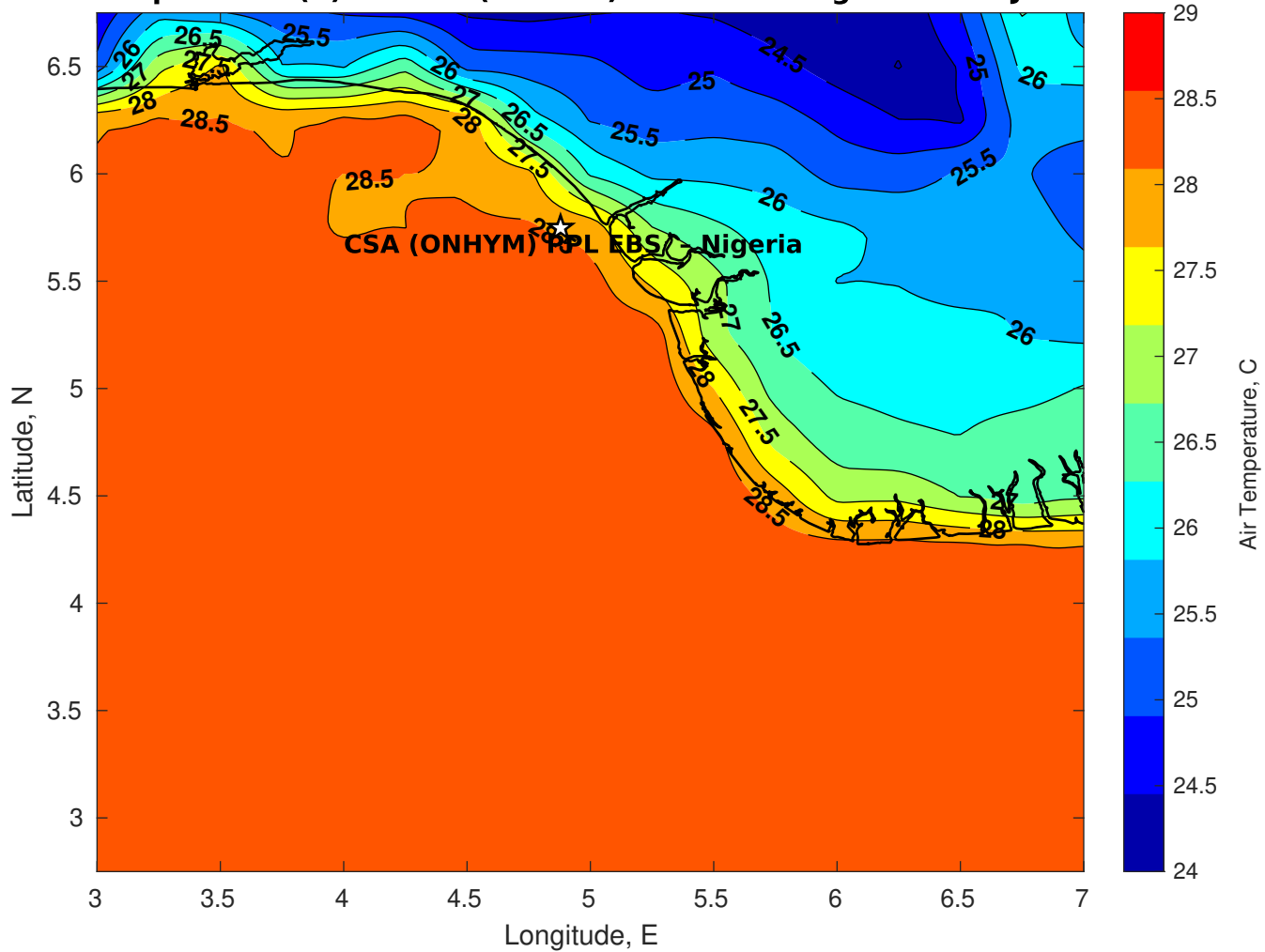
Air Temperature (C) for CSA (ONHYM) PPL EBS - Nigeria at 25-Jan-2026
