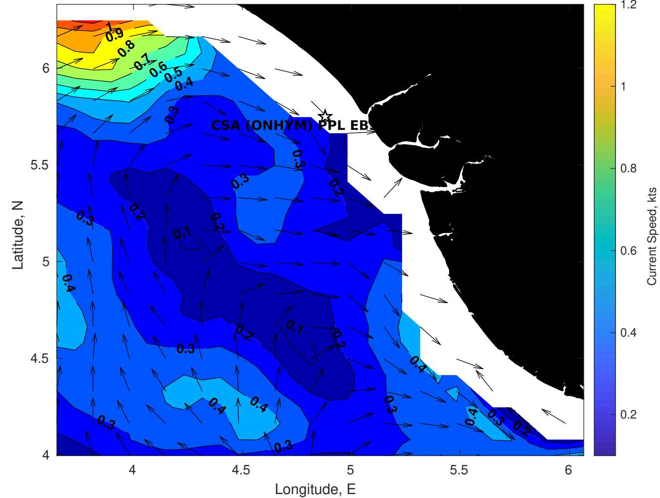
Surface Currents for CSA (ONHYM) PPL EBS - Nigeria at 24-Jan-2026 00:00:00
