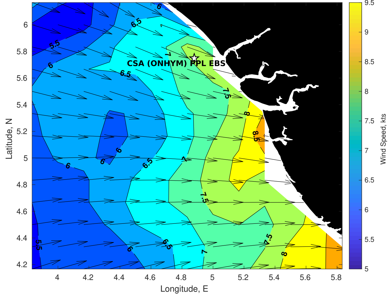
GFS Winds (kts) for CSA (ONHYM) PPL EBS - Nigeria at 25-Jan-2026 09:00:00
