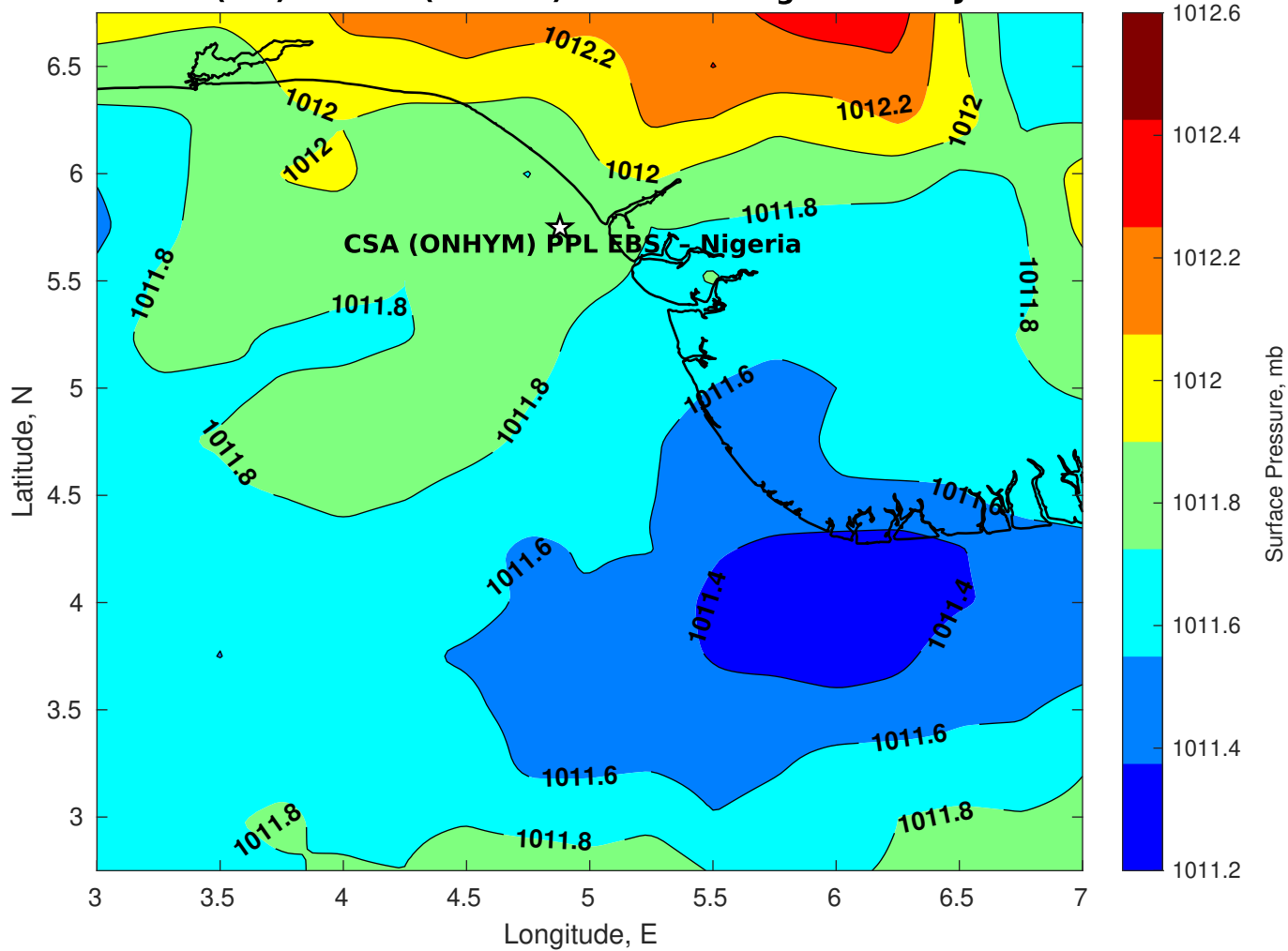
Surface Pressure (mb) for CSA (ONHYM) PPL EBS - Nigeria at 25-Jan-2026 06:00:00
