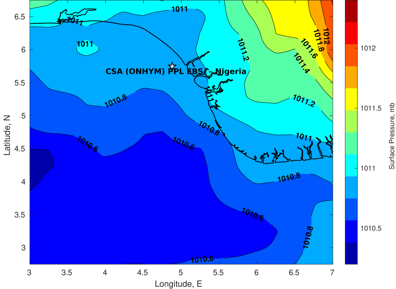
Surface Pressure (mb) for CSA (ONHYM) PPL EBS - Nigeria at 27-Jan-2026 06:00:00
