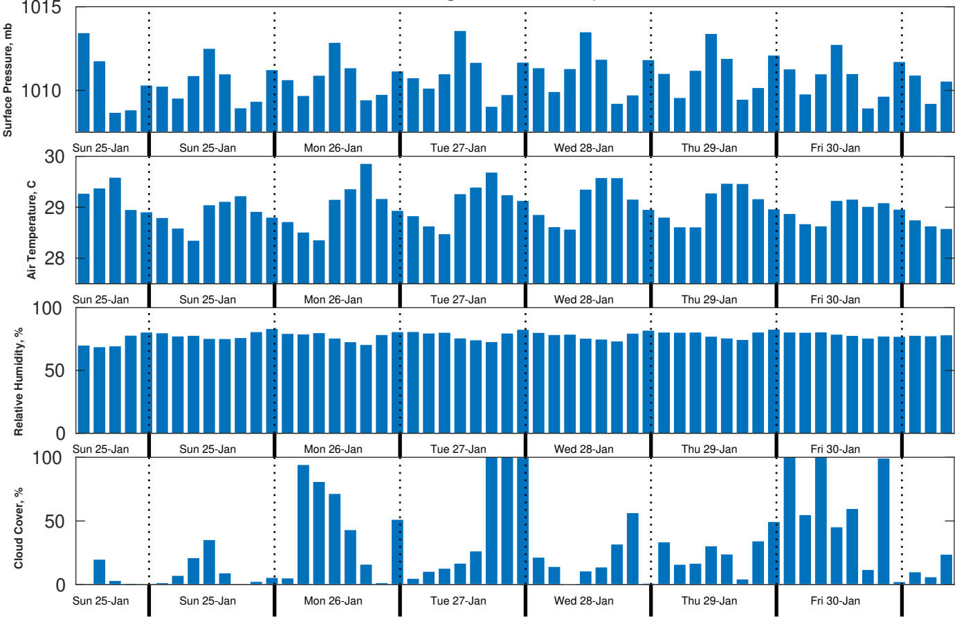
Met Forecast for CSA (ONHYM) PPL EBS - Nigeria from 25-Jan-2026 06:00:00 to 01-Feb-2026 06:00:00
