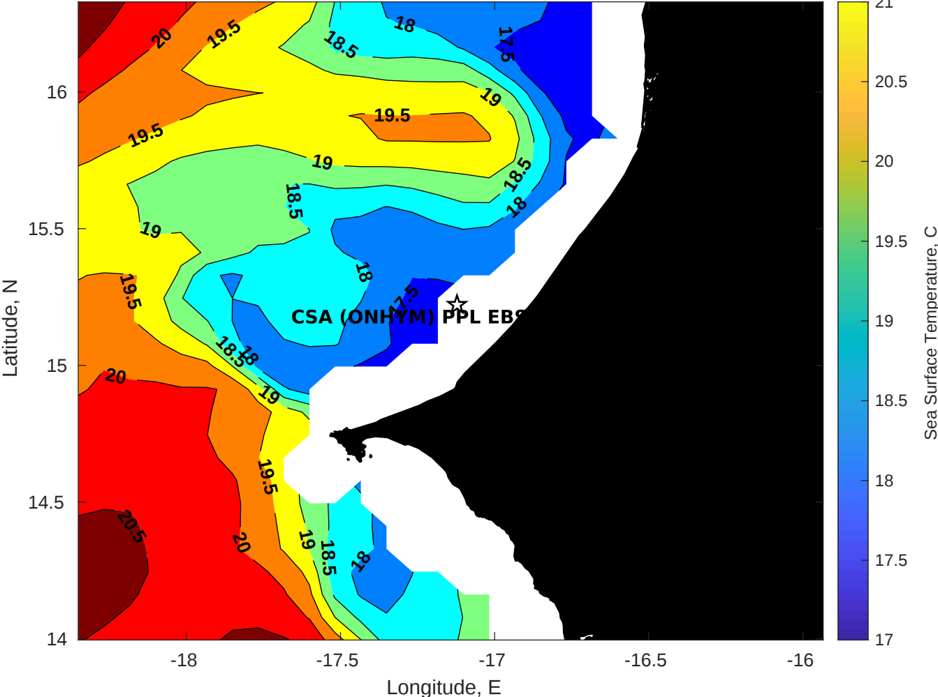
SST for CSA (ONHYM) PPL EBS - Senegal at 24-Jan-2026 00:00:00
