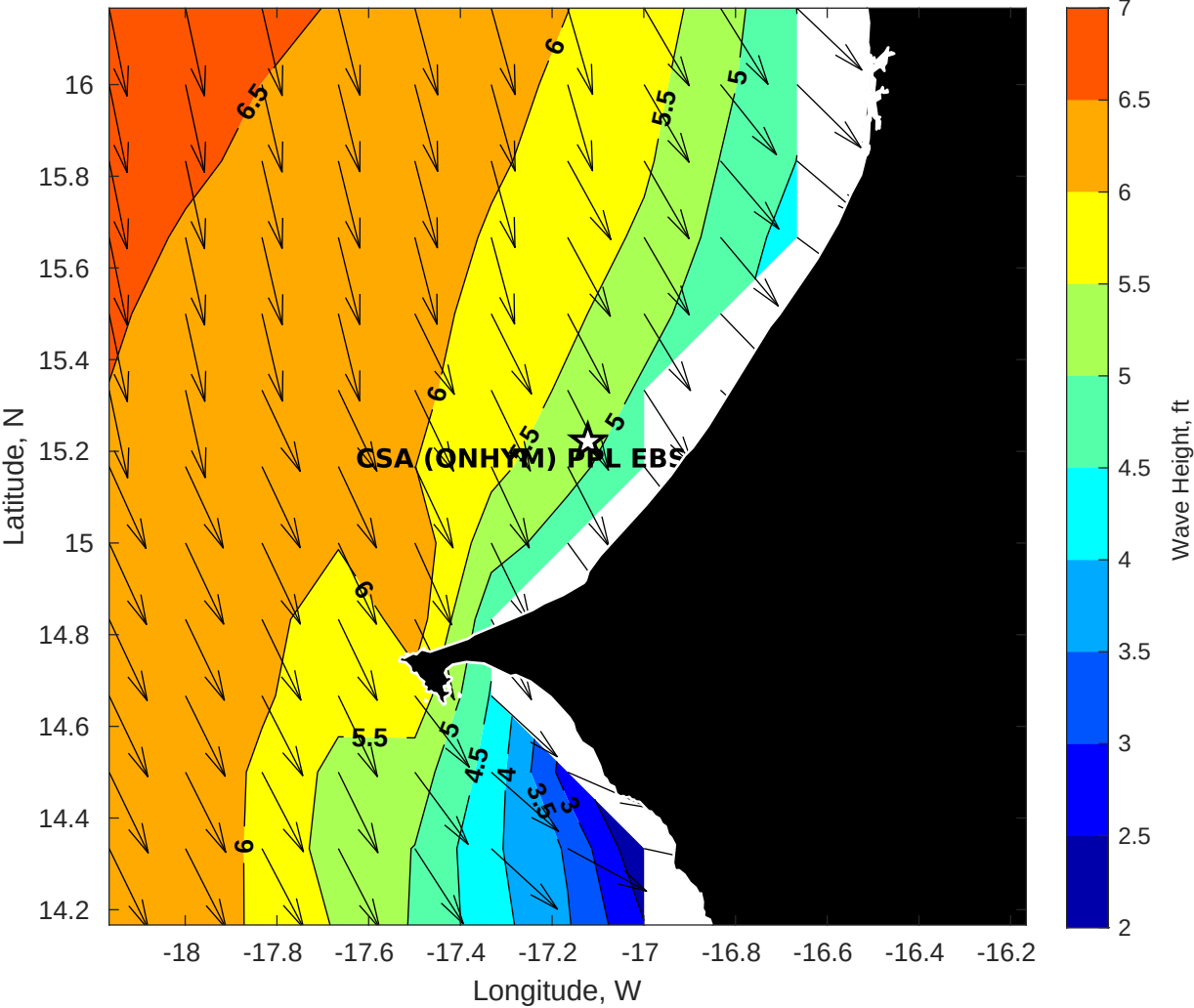
GFS Wave Height (ft) for CSA (ONHYM) PPL EBS - Senegal at 25-Jan-2026 09:00:00
