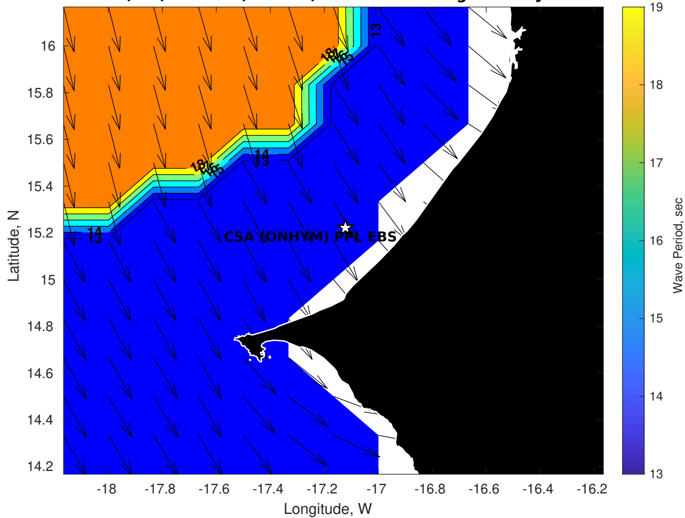
GFS Wave Period (sec) for CSA (ONHYM) PPL EBS - Senegal at 25-Jan-2026 09:00:00
