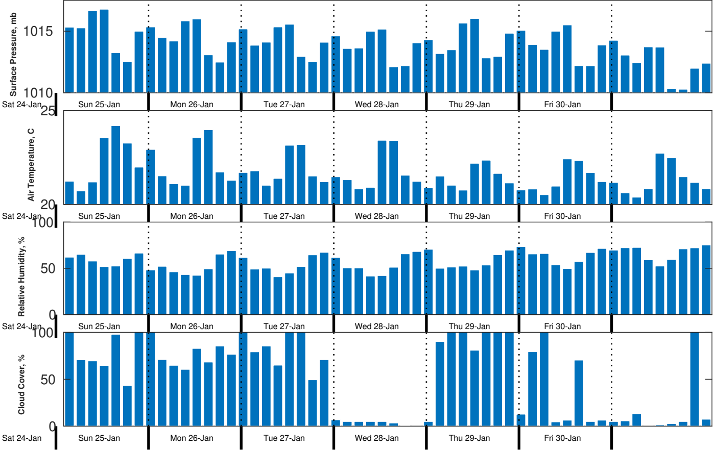
Met Forecast for CSA (ONHYM) PPL EBS - Senegal from 25-Jan-2026 00:00:00 to 01-Feb-2026 00:00:00
