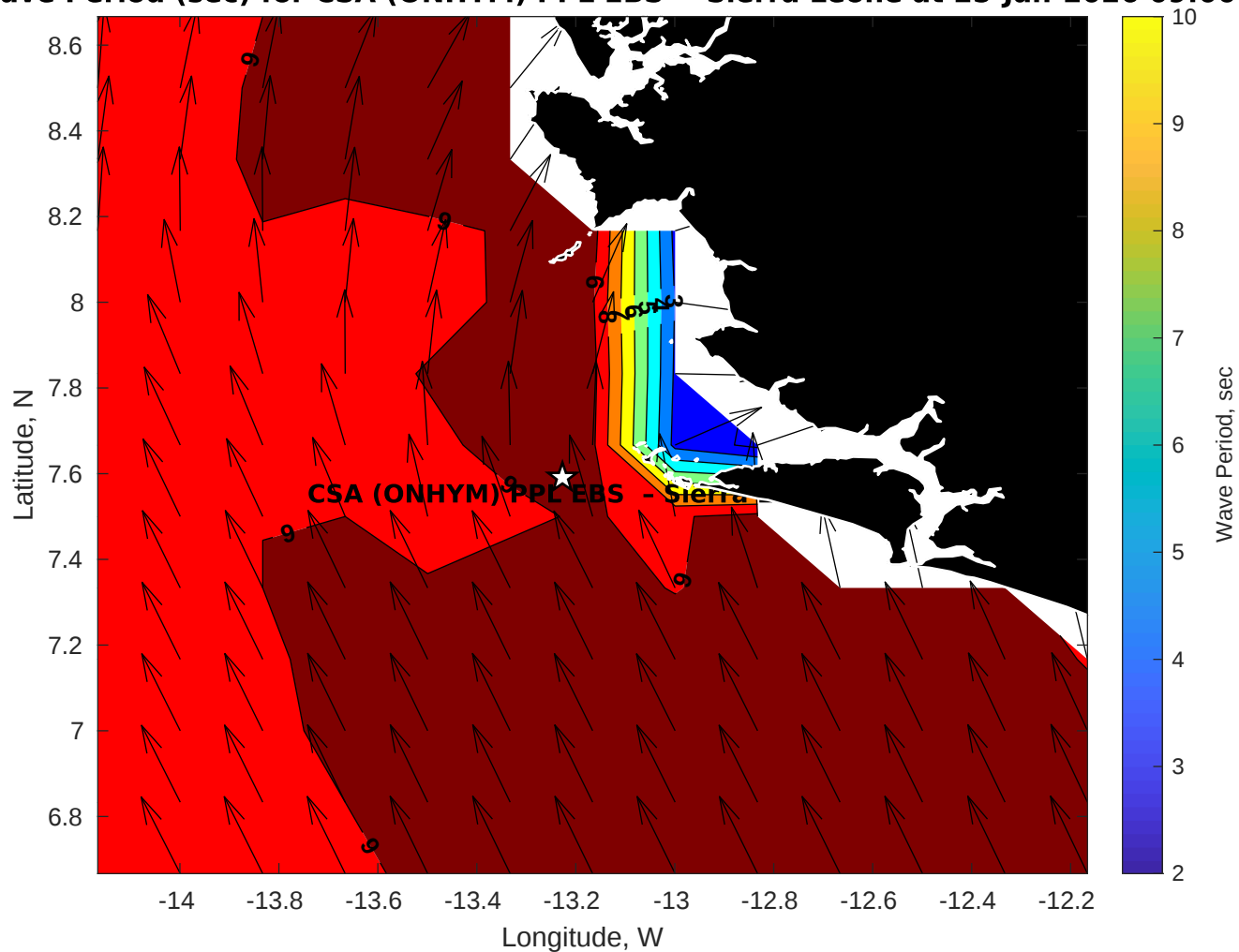
GFS Wave Period (sec) for CSA (ONHYM) PPL EBS - Sierra Leone at 25-Jan-2026 09:00:00
