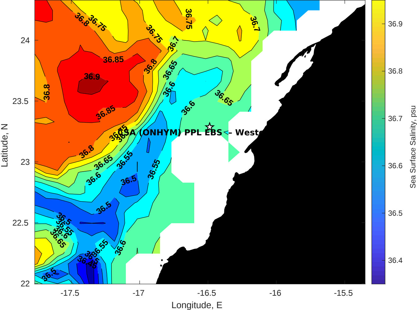
Surface Salinity for CSA (ONHYM) PPL EBS - Western Sahara at 24-Jan-2026 00:00:00
