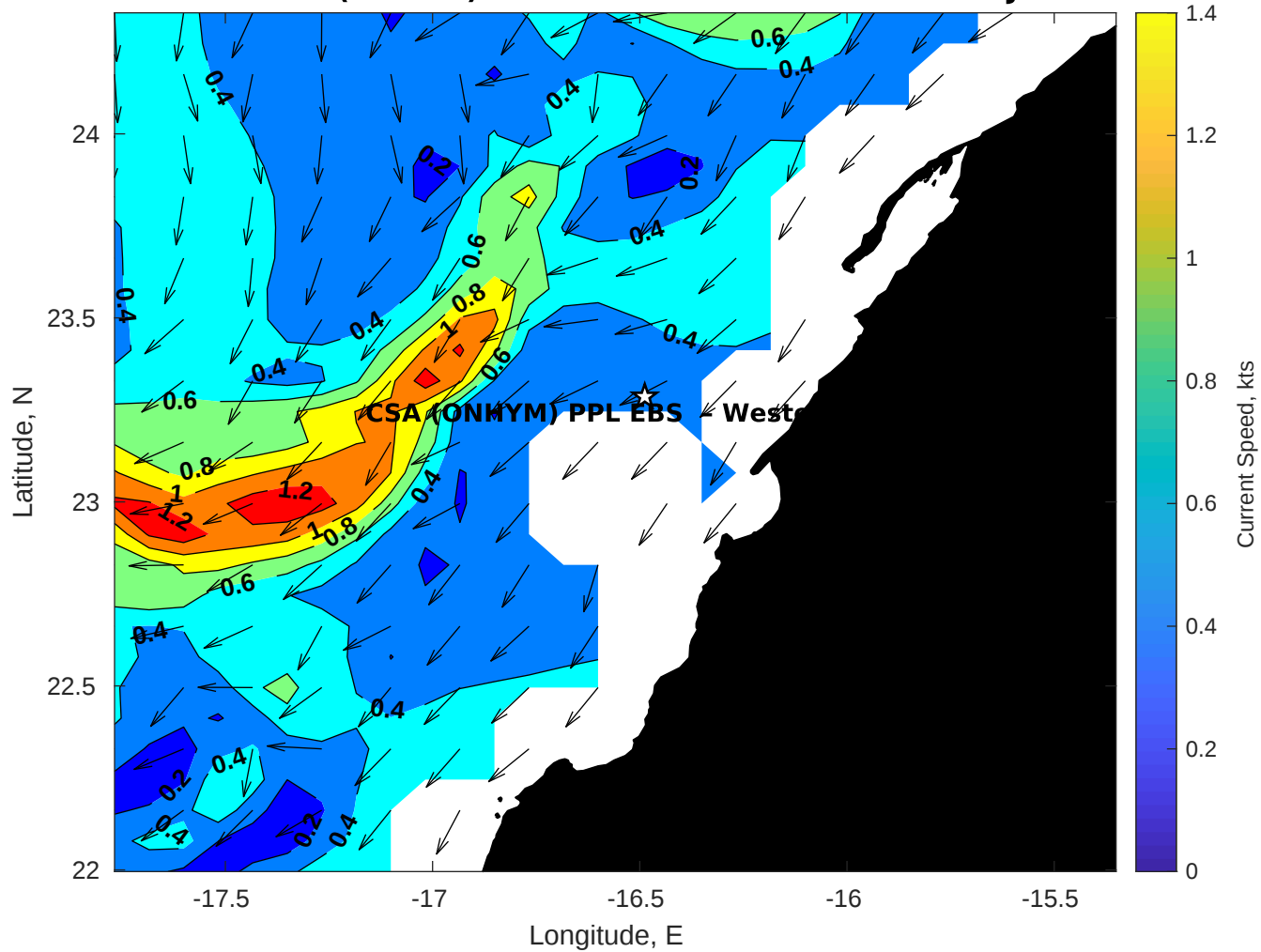
Surface Currents for CSA (ONHYM) PPL EBS - Western Sahara at 24-Jan-2026 00:00:00
