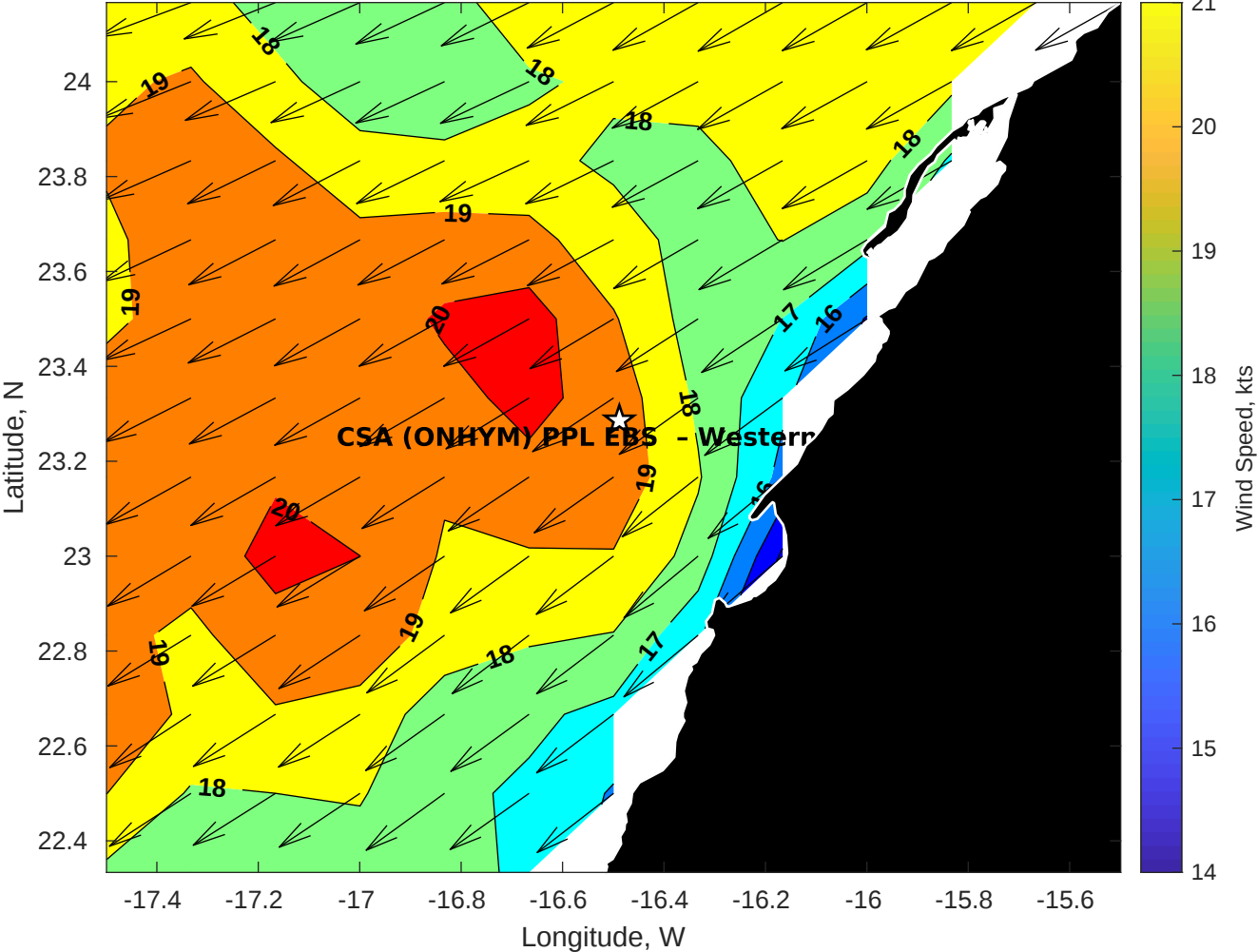
GFS Winds (kts) for CSA (ONHYM) PPL EBS - Western Sahara at 25-Jan-2026 09:00:00
