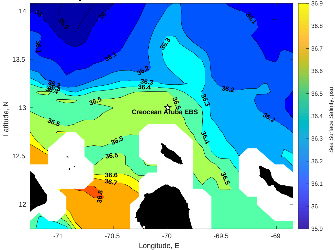
Surface Salinity for Creocan Aruba EBS at 24-Jan-2026 00:00:00
