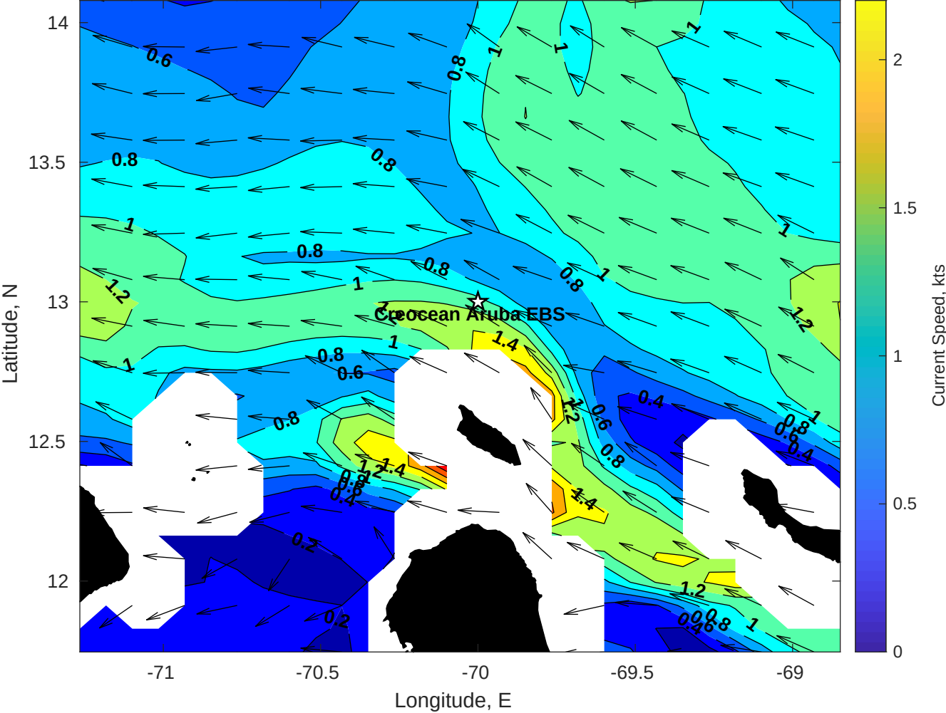
Surface Currents for Creocean Aruba EBS at 24-Jan-2026 00:00:00
