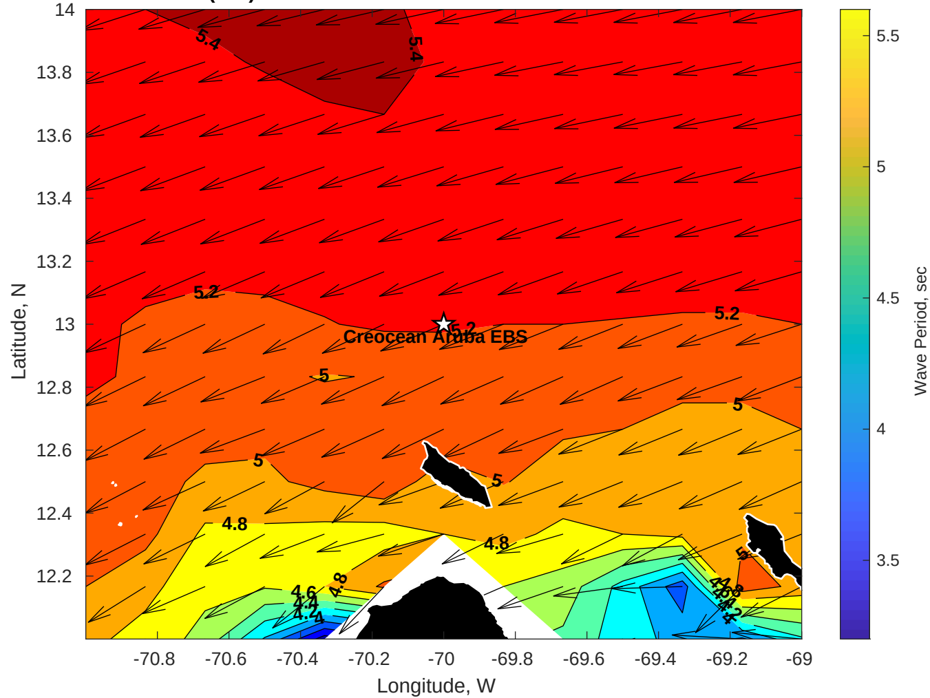
GFS Wave Period (sec) for Creoccean Aruba EBS at 25-Jan-2026 09:00:00
