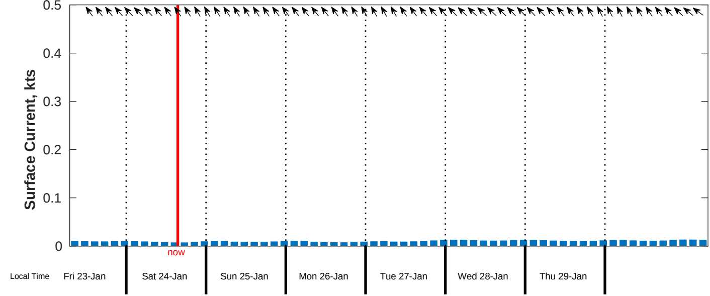
Surface Current Forecast for Creocean Aruba EBS from 24-Jan-2026 00:00:00 to 01-Feb-2026 00:00:00
