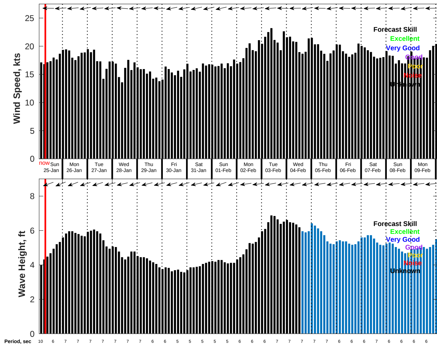
Wind & Wave Forecast for Creocan Aruba EBS from 25-Jan-2026 02:00:00 to 10-Feb-2026 02:00:00
