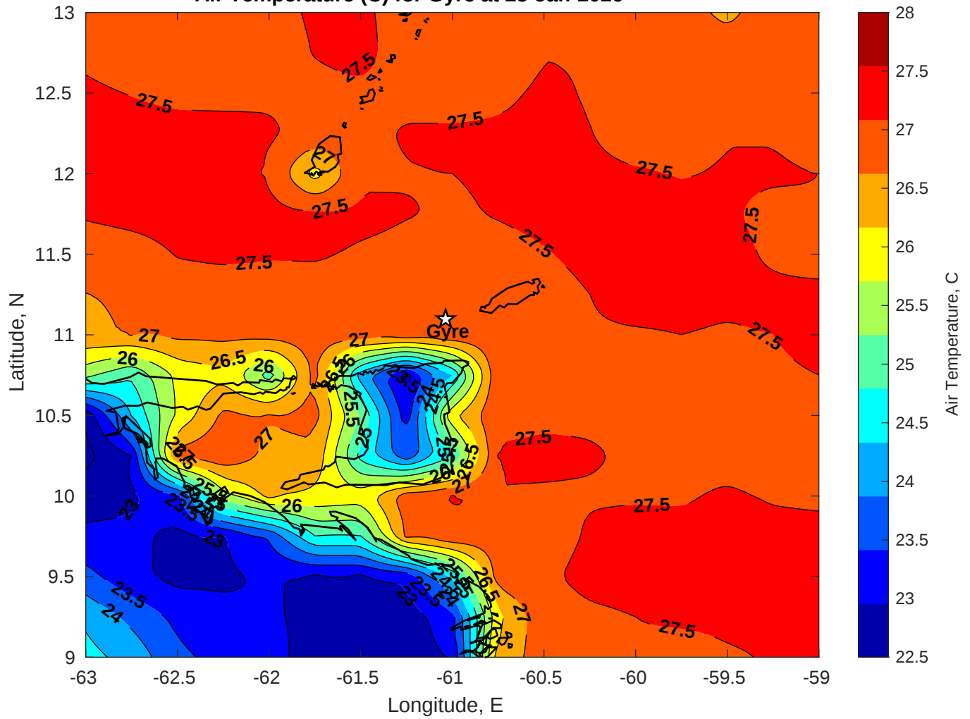
Air Temperature (C) for Gyre at 25-Jan-2026
