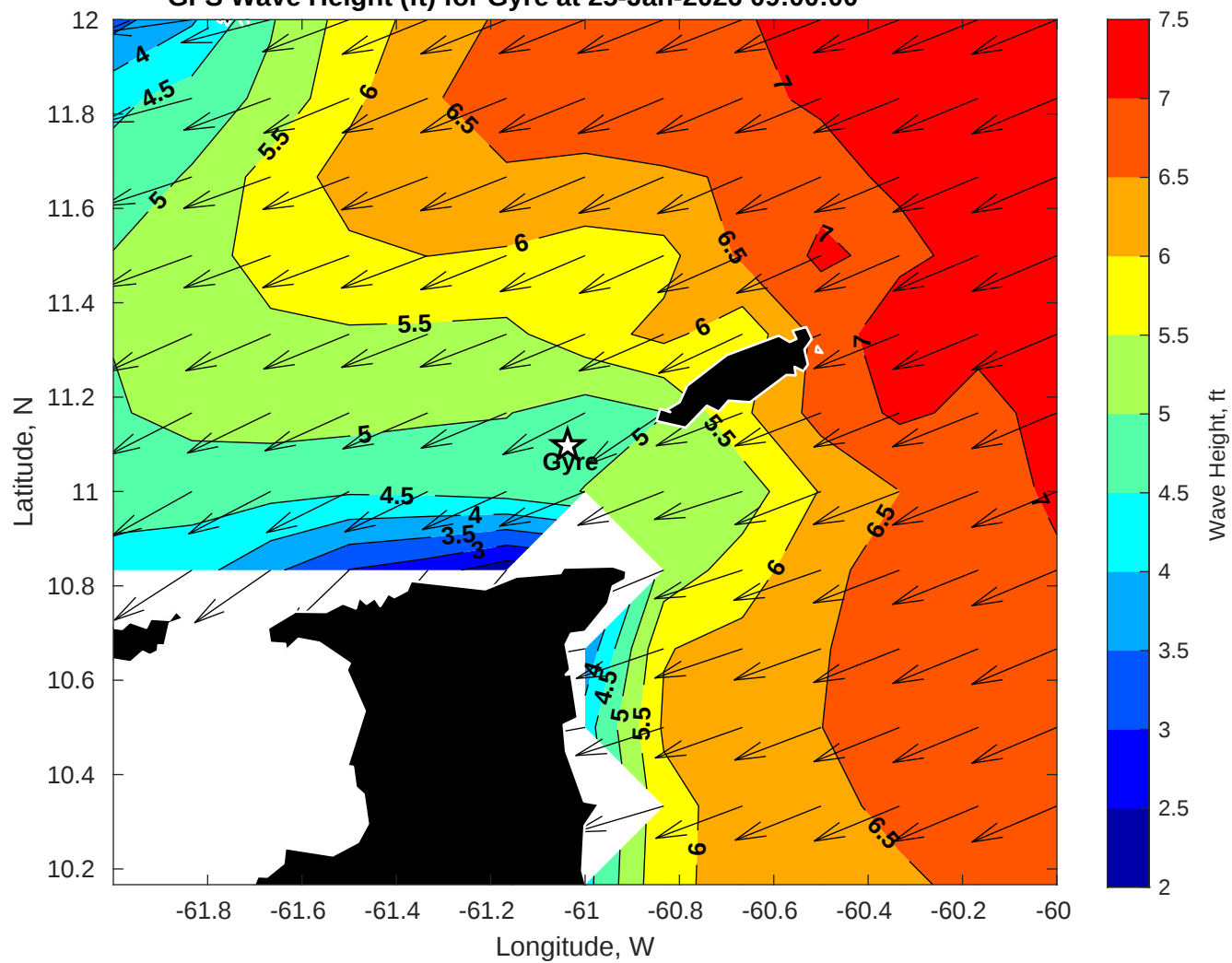
GFS Wave Height (ft) for Gyre at 25-Jan-2026 09:00:00
