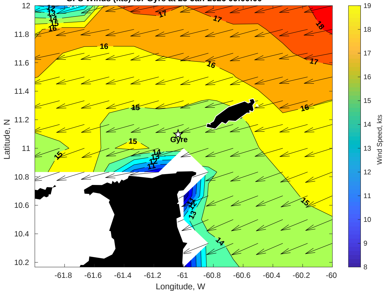
GFS Winds (kts) for Gyre at 25-Jan-2026 09:00:00
