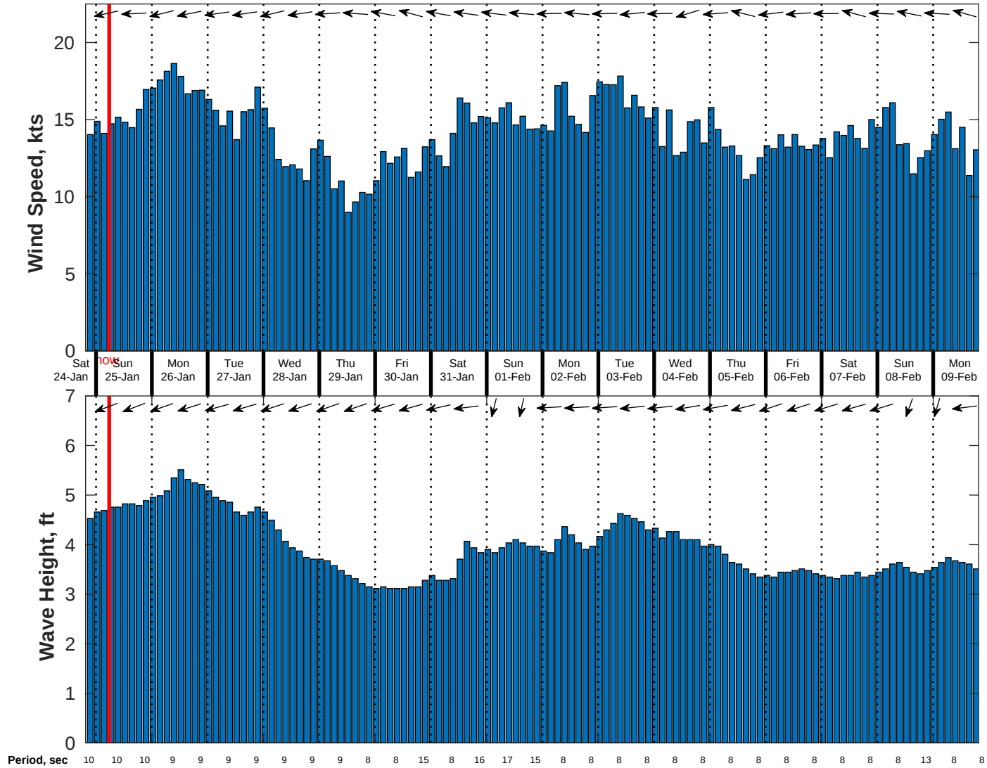
Wind & Wave Forecast for Gyre from 24-Jan-2026 20:00:00 to 09-Feb-2026 20:00:00
