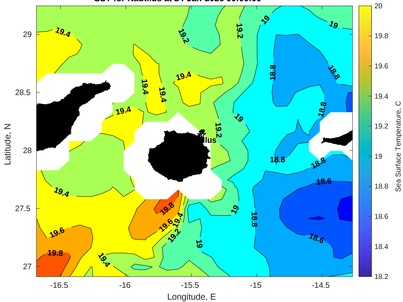
SST for Nautilus at 24-Jan-2026 00:00:00
